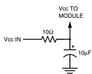
Figure 41: Supply Filter
