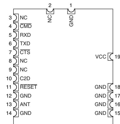
Figure 5: DTS Series Transceiver Pin Assignments (Top View)
