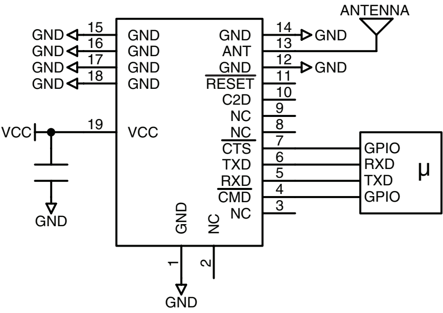
Figure 40: DTS Series Transceiver Basic Application Circuit
