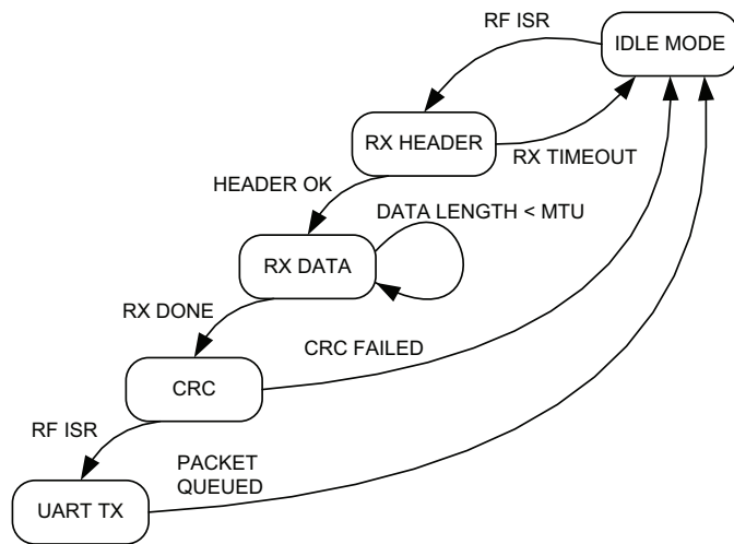
Figure 8: DTS Series Transceiver Receiver State Diagram
