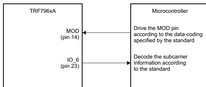
Figure 6-28. Control of RF Modulation Using MOD
