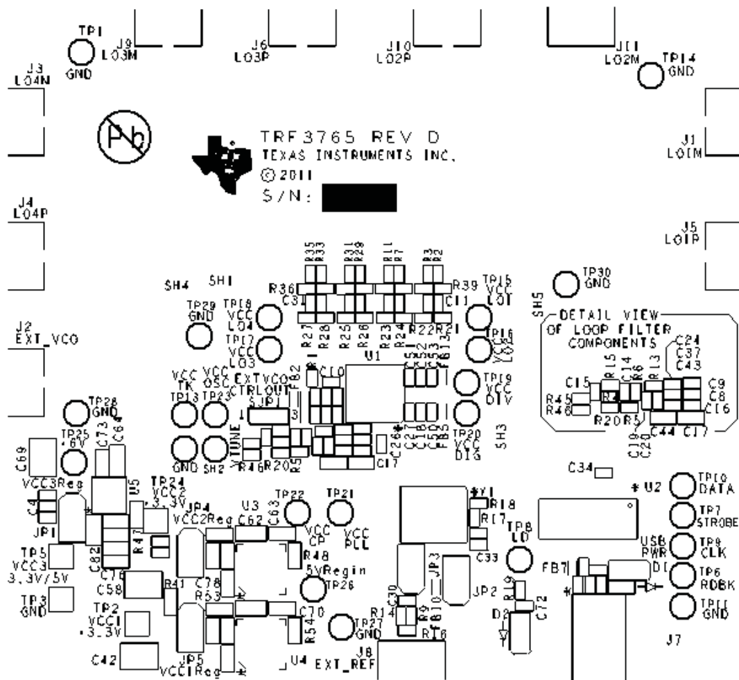
Figure 5. Silkscreen, Top
