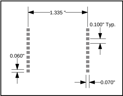
Figure 6: Recommended pad layout
