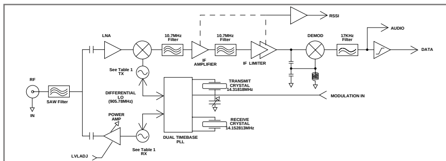
Figure 7: SC-S Series Block Diagram
