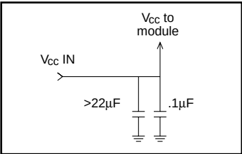
Figure 8: Suggested supply filter
