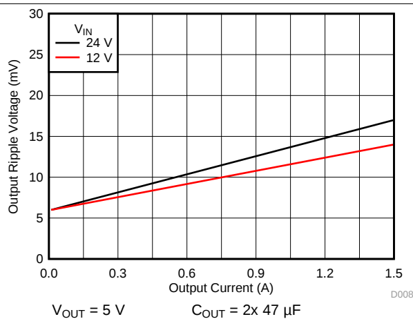
Figure 8. Ripple Voltage vs Output Current
