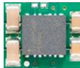
RLF Package and Typical Layout
