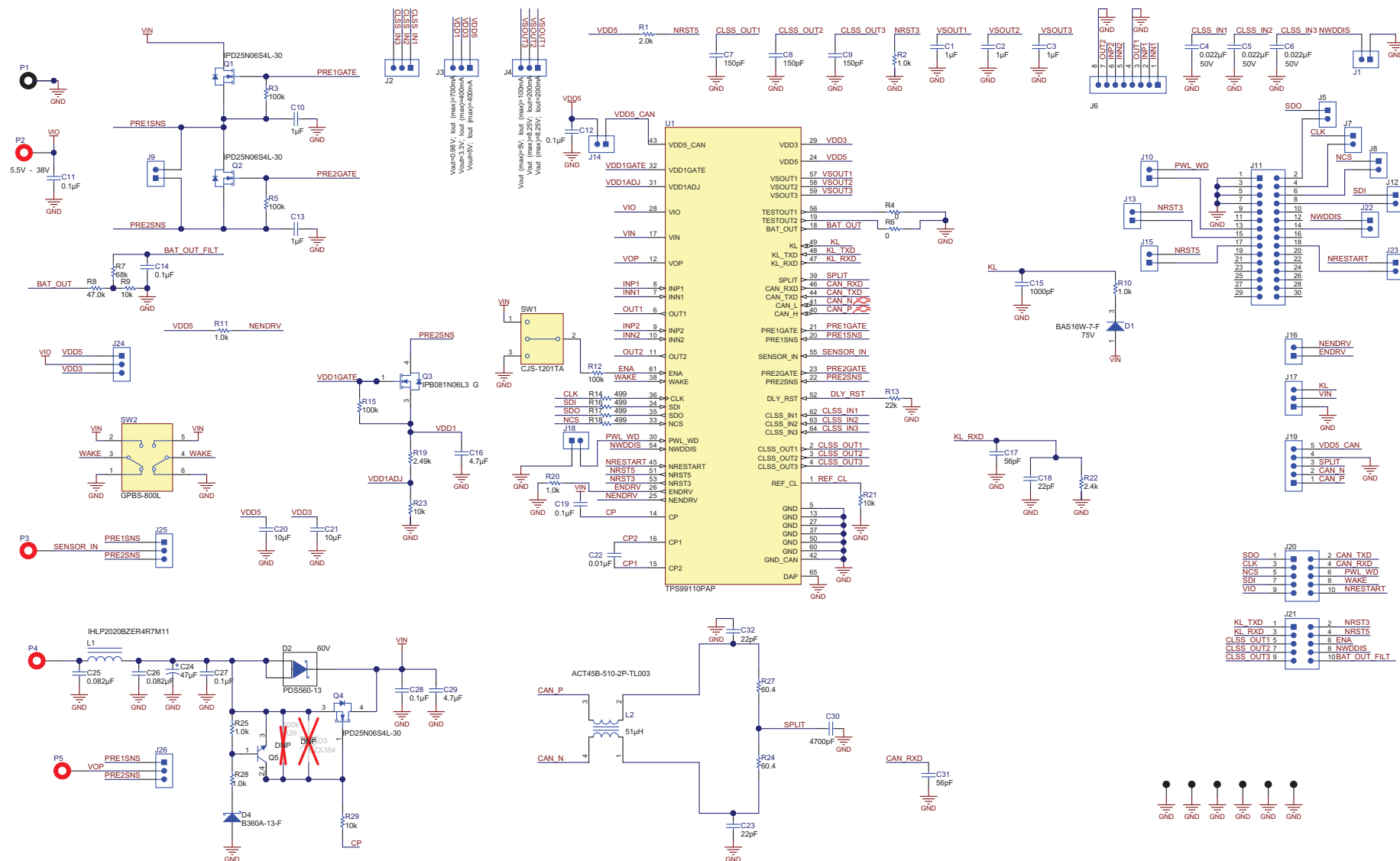
Figure 5. TPS99110EVM Schematic
