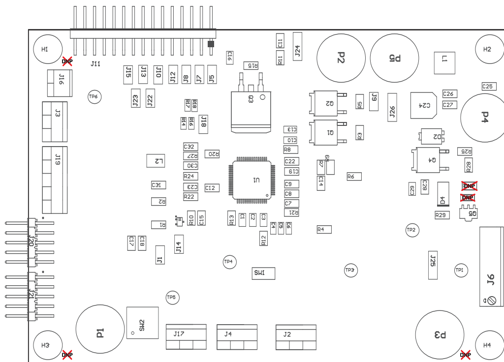
Figure 6. Top-Side Layer
