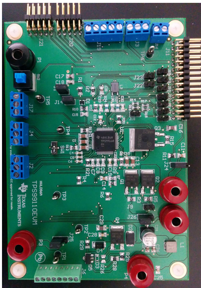
Figure 1. TPS99110EVM Board
