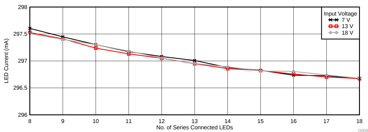
Figure 10. Output LED Current vs LED String Configuration ( V_{IADJ} = 1.26 \text{ V} )
