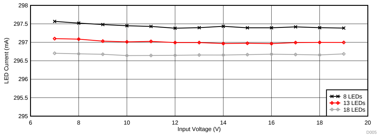
Figure 7. Output LED Current vs Input Voltage ( V_{IADJ} = 1.26 \text{ V} )
