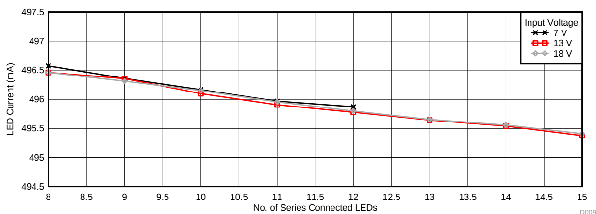
Figure 11. Output LED Current vs LED String Configuration ( V_{IADJ} = 2.1 \text{ V} )
