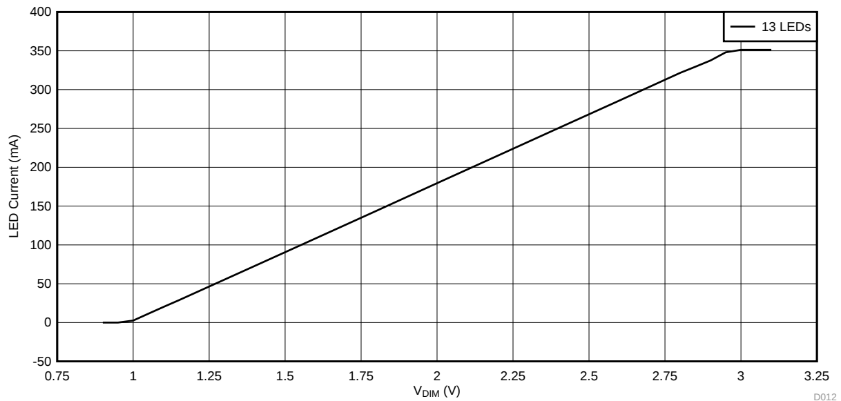
Figure 13. LED Current vs DIM/PWM Voltage ( V_{IADJ} = 1.49 V, Number of LEDs in Series = 13)
