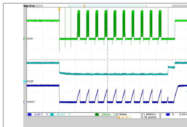
Figure 27. LED Short-Circuit Fault
