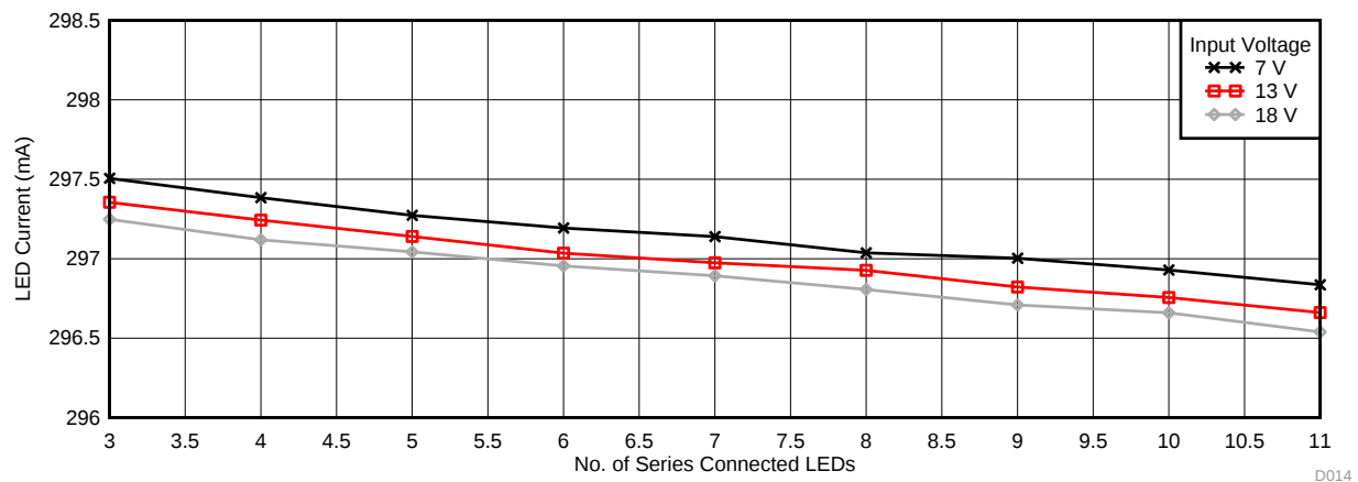
Figure 26. Output LED Current vs LED String Configuration ( V_{IADJ} = 1.26\text{ V} )
