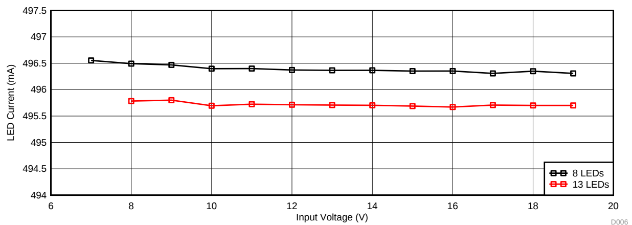
Figure 8. Output LED Current vs Input Voltage ( V_{IADJ} = 2.1 \text{ V} )
