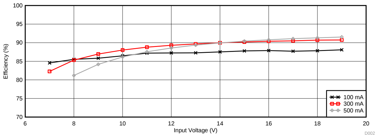
Figure 4. Efficiency vs Input Voltage (Number of Series-Connected LEDs = 13)
