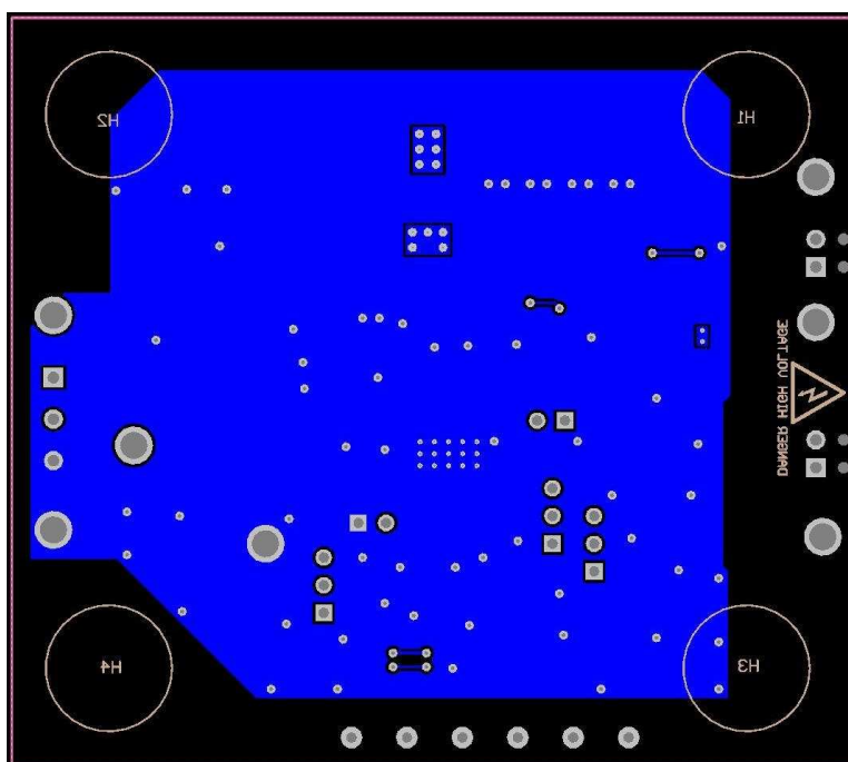
Figure 31. Bottom Layer and Bottom Overlay (Bottom View)
