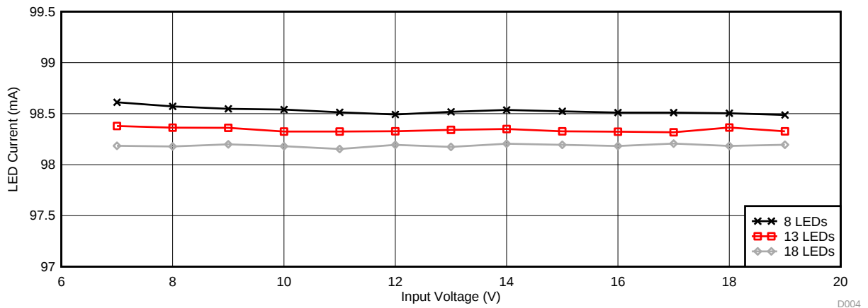
Figure 6. Output LED Current vs Input Voltage ( V_{IADJ} = 420 \text{ mV} )
