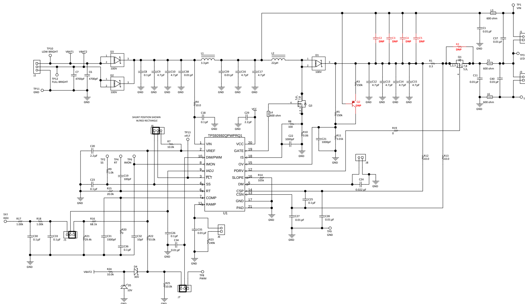
Figure 2. TPS92692EVM-880 Schematic: Configured as a Boost LED Driver
