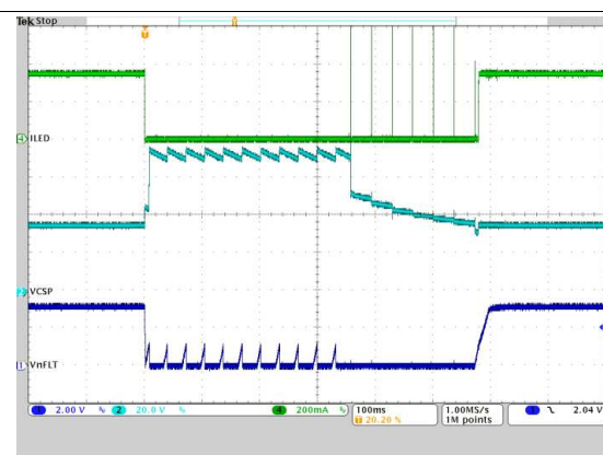
Figure 28. LED Open-Circuit Fault
