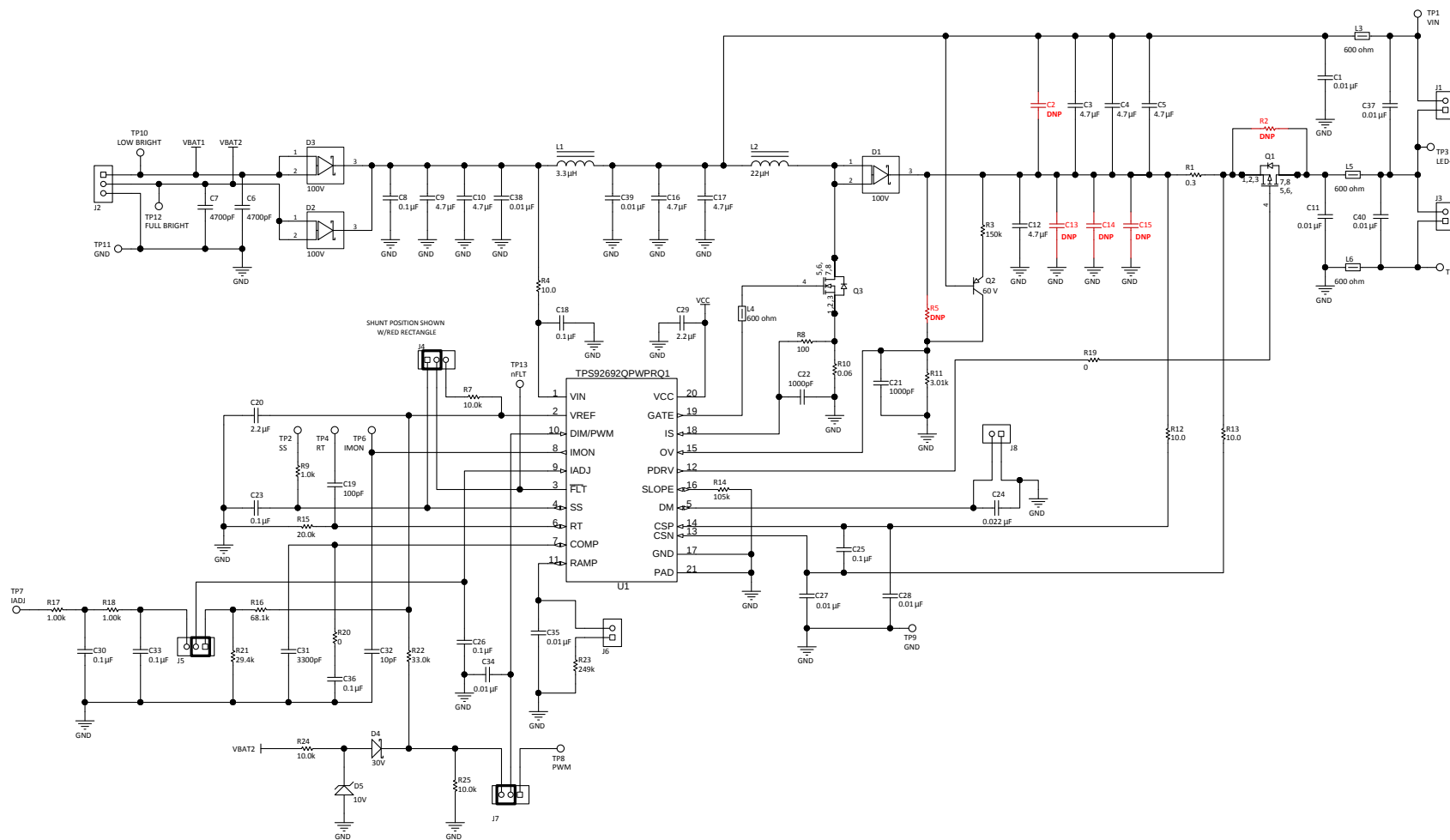
Figure 23. TPS92692EVm-880 Schematic: Configured as a Buck-Boost LED Driver
