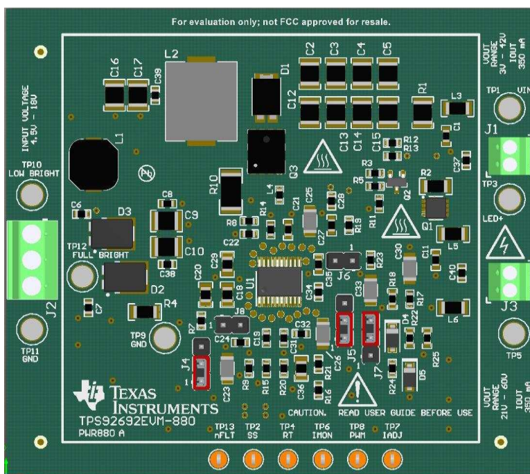
Figure 29. Assembly Drawing
