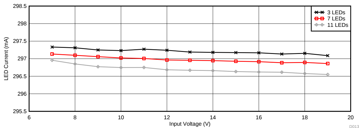
Figure 25. Output LED Current vs Input Voltage ( V_{IADJ} = 1.26 V)
