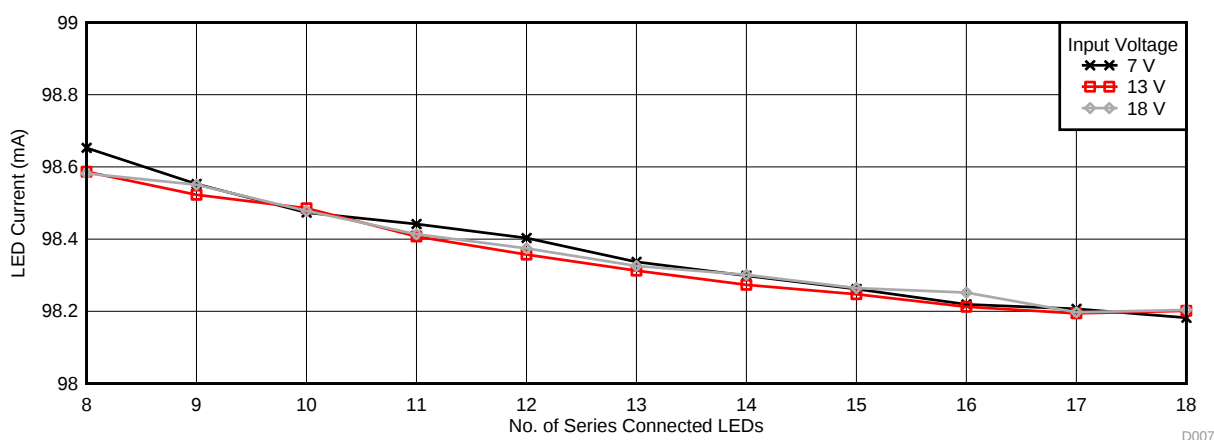
Figure 9. Output LED Current vs LED String Configuration ( V_{IADJ} = 420 \text{ mV} )
