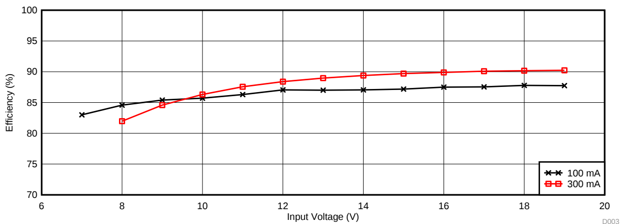
Figure 5. Efficiency vs Input Voltage (Number of Series-Connected LEDs = 18)
