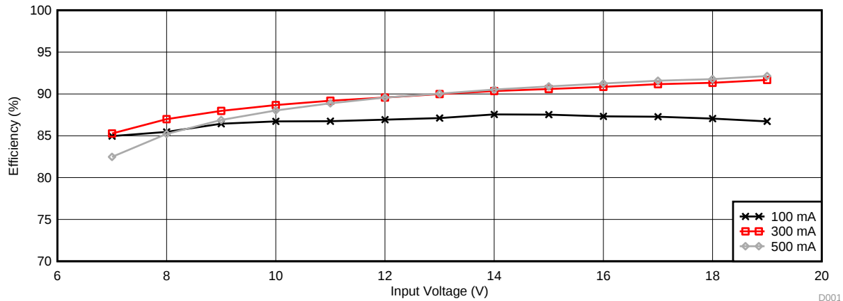
Figure 3. Efficiency vs Input Voltage (Number of Series-Connected LEDs = 8)
