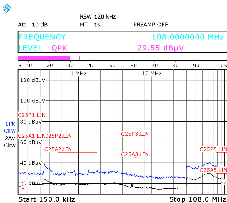
Figure 22. Conducted EMI Based on CISPR 25 Class 3 Limits (Dither Modulation Enabled)
