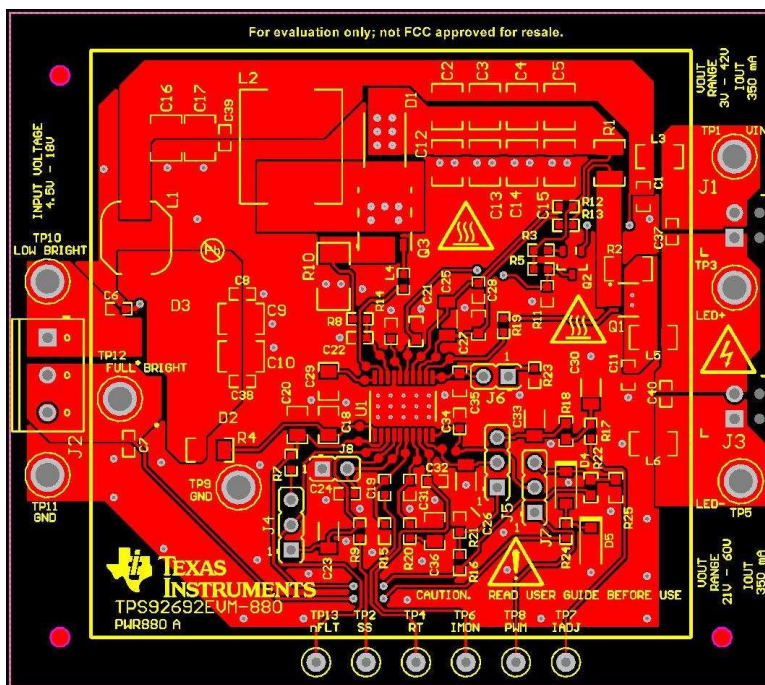
Figure 30. Top Layer and Top Overlay (Top View)
