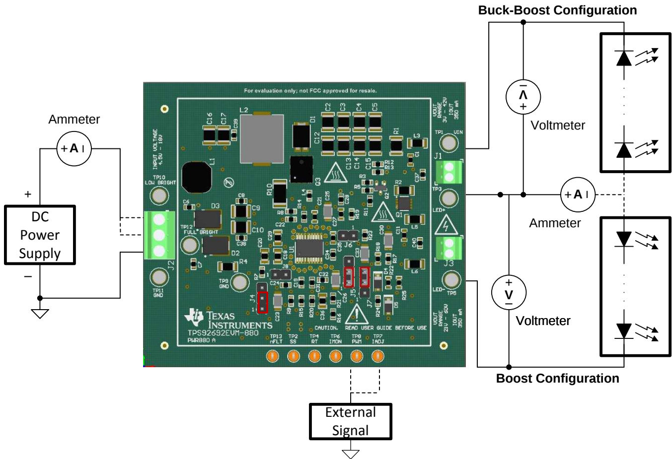
Figure 1. Connection Diagram
