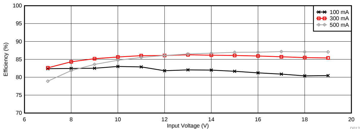
Figure 24. Efficiency vs Input Voltage (Number of Series-Connected LEDs = 7)
