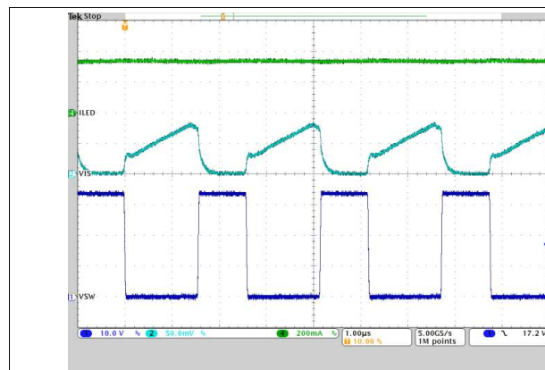
Ch1: Switch node voltage Ch2: Switch current sense voltage Ch4: LED current; Time: 1 \mu s/div
