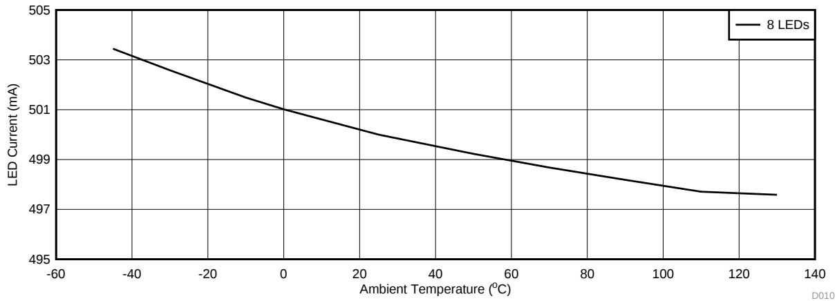
Figure 12. LED Current vs Ambient Temperature ( V_{IN} = 13 V, Number of LEDs in Series = 8)
