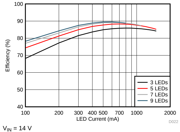
Figure 56. Efficiency
