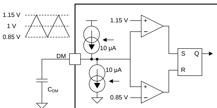
Figure 22. Frequency Dither Operation
