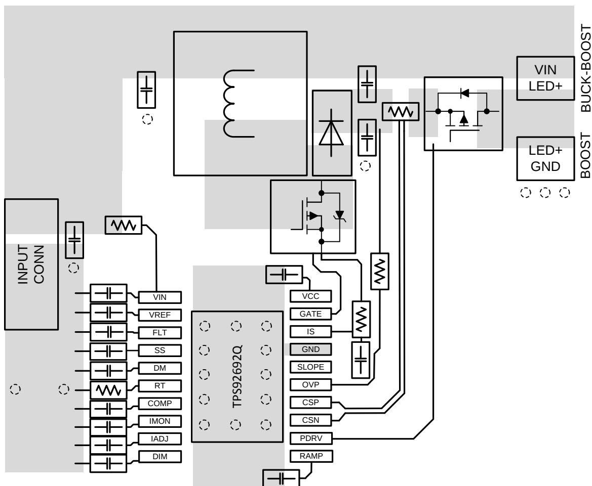
Figure 59. Layout Recommendation
