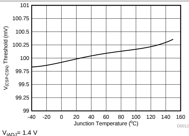
Figure 13. V_{(CSP-CSN)} Threshold vs Junction Temperature
