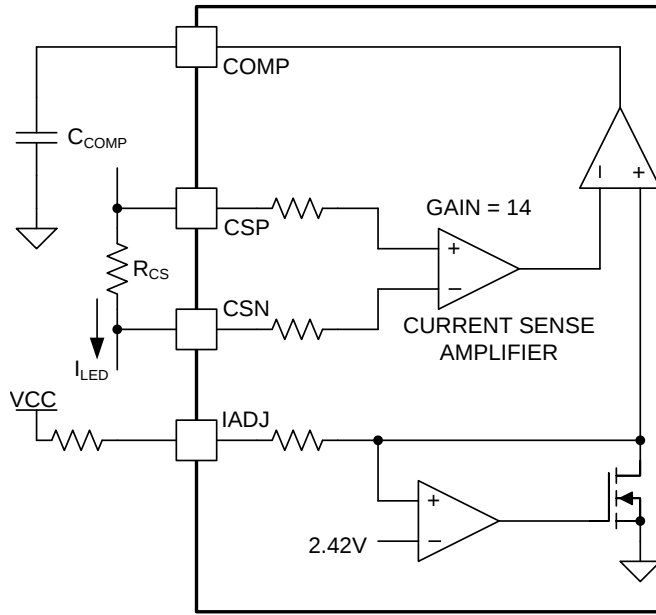
Figure 41. Integral Compensator
