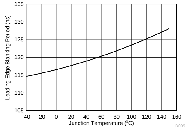
Figure 10. Leading Edge Blanking Period vs Junction Temperature
