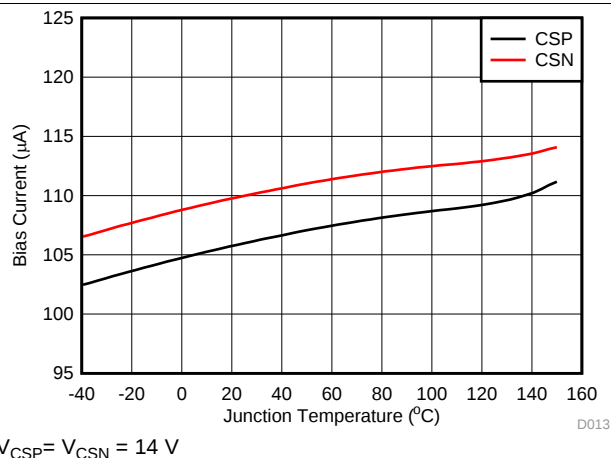
Figure 14. CSP/CSN Input Bias Current vs Junction Temperature
