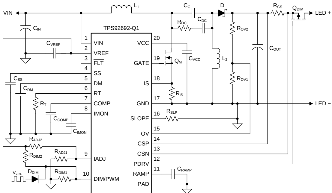
Figure 38. SEPIC LED Driver
