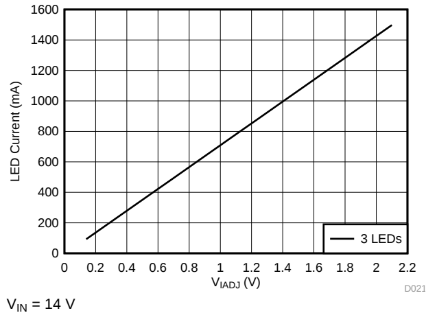
Figure 55. LED Current vs IADJ Voltage
