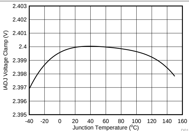
Figure 18. V_{IADJ} Voltage Clamp vs Junction Temperature
