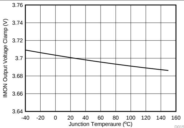
Figure 16. V_{IMON(CLP)} vs Junction Temperature
