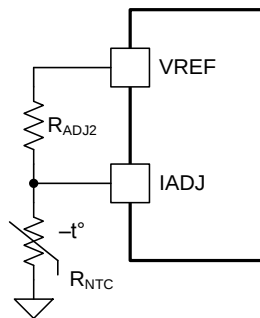
Figure 27. Thermal Fold-back Circuit Using External NTC Resistor
