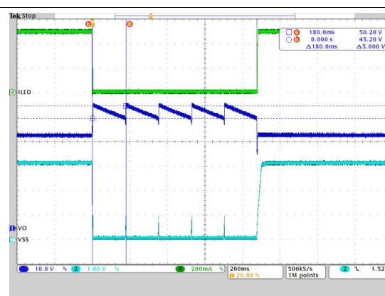
Ch1: Output voltage; Ch2: Soft-start (SS) voltage; Ch4: LED current; Time: 200 ms/div
