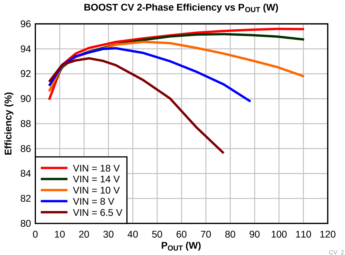
Figure 2. Efficiency vs Output Power
