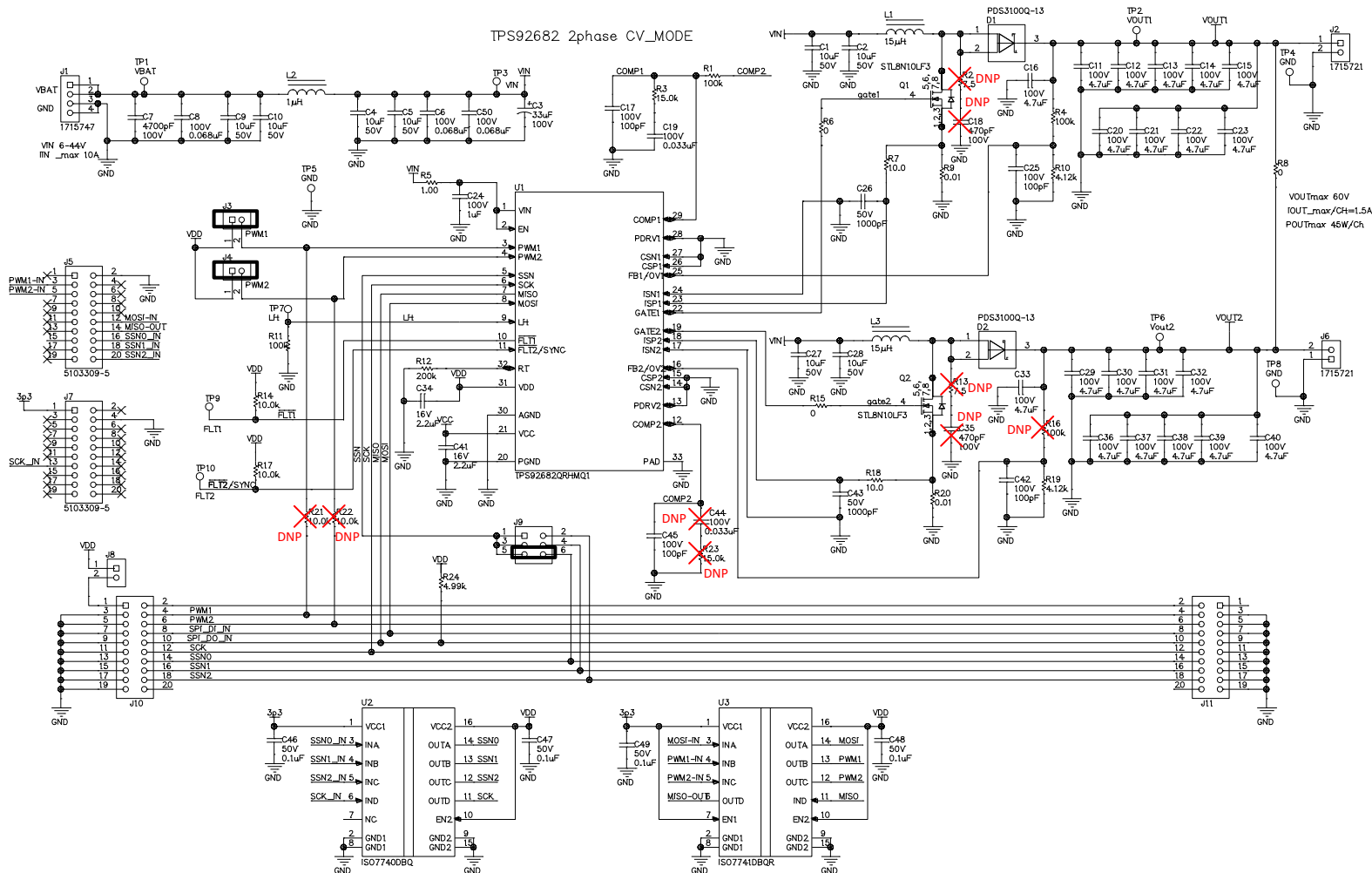
Figure 7. TPS92682EVM-069 Schematic
