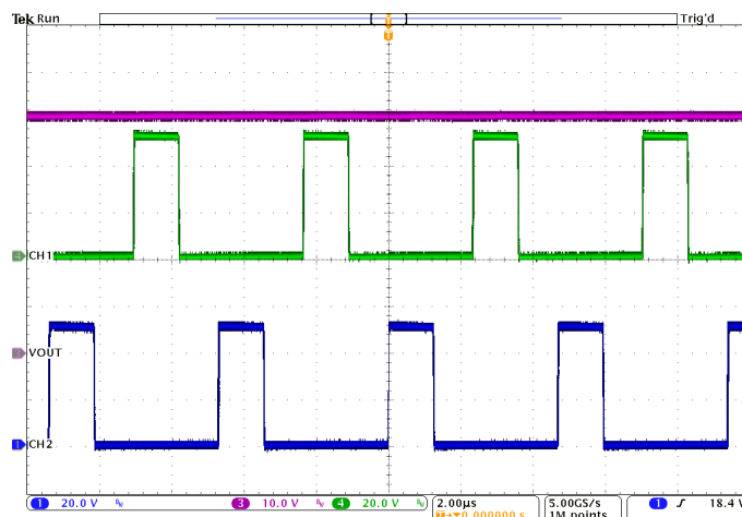
Figure 3. CV boost 2-phase SW-node voltage
