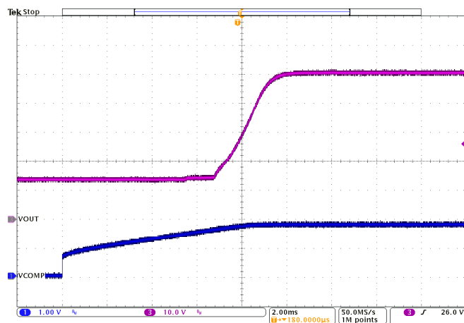
Figure 4. Soft-start timing
