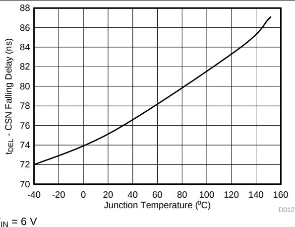
Figure 5. CSN Pin Falling Delay Time vs. Junction Temperature
