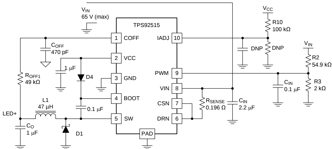
Figure 33. Application Schematic
