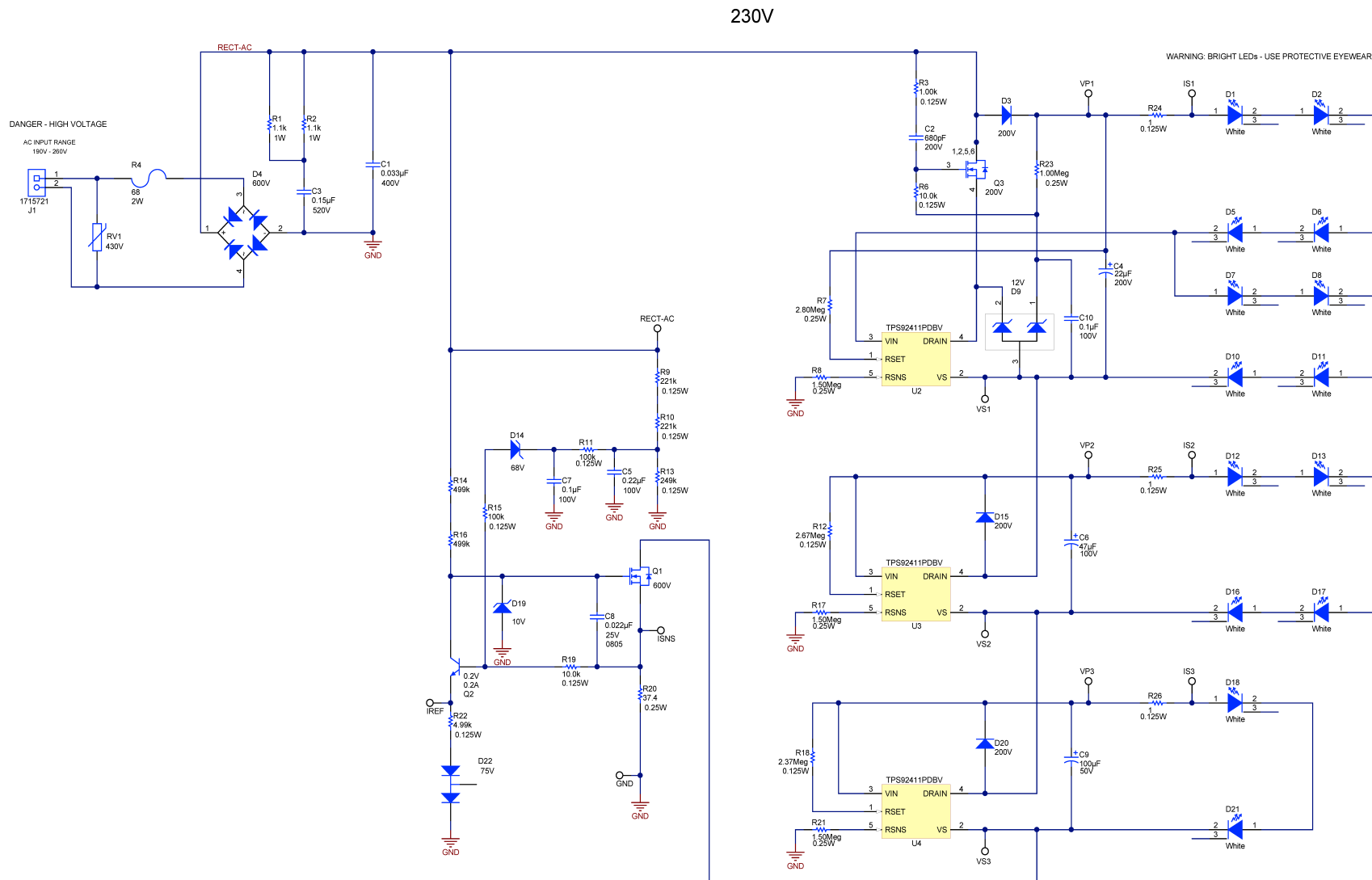
Figure 1. TPS92411EVM-002 Schematic
