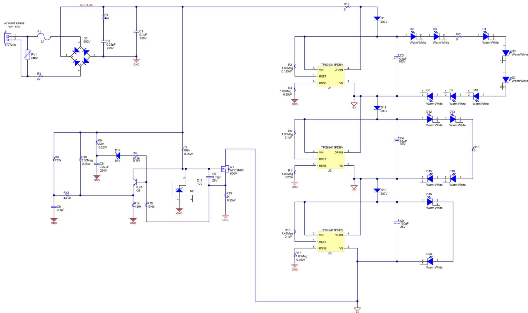
Figure 1. TPS92411EVM-001 Schematic
