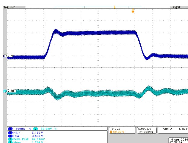
Figure 25. Line Transient Response for TPS8268180 (Vout = 1.80V; Iout = 800mA, Vin = 4V to 5V to 4V)
