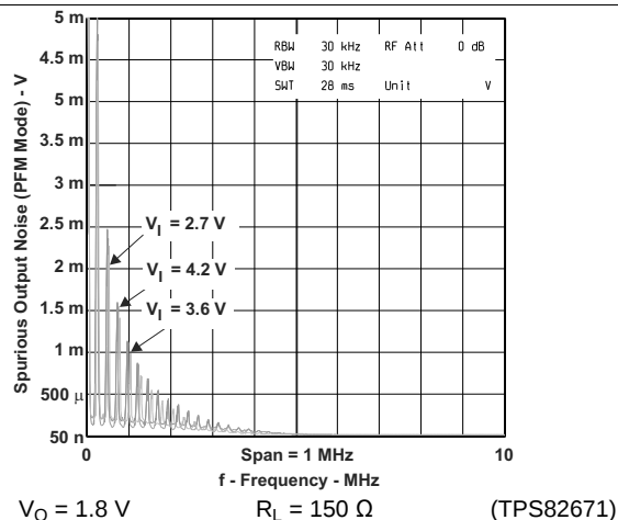
Figure 4. Spurious Output Noise (PFM Mode) vs. Frequency
