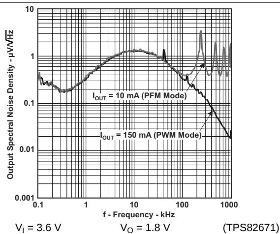
Figure 6. Output Spectral Noise Density vs. Frequency
