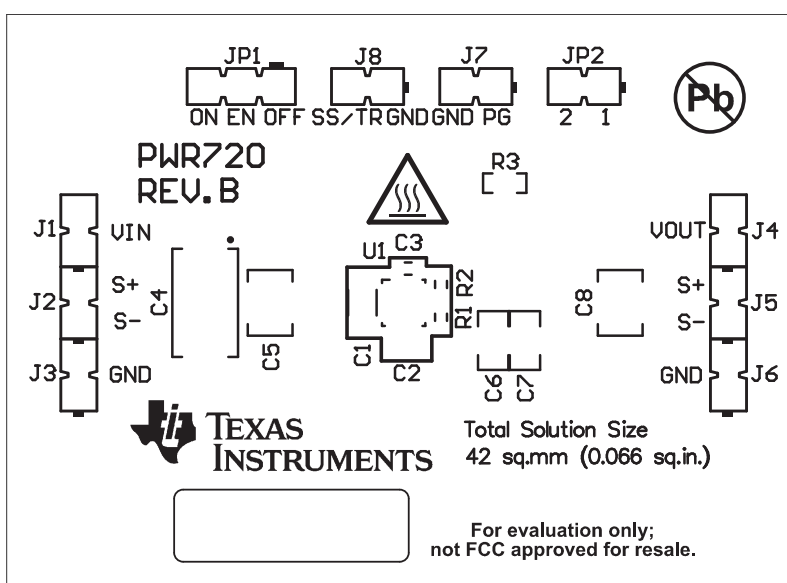
Figure 2. Top Overlay
