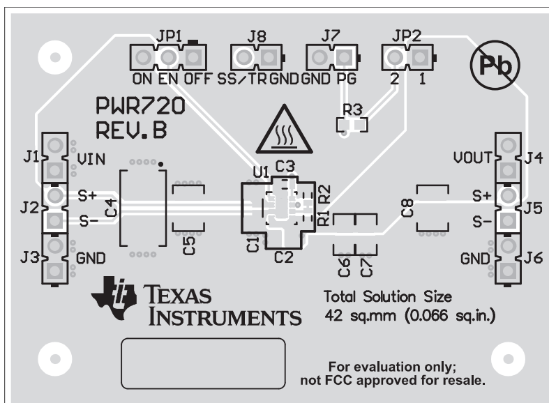
Figure 1. Top Assembly
