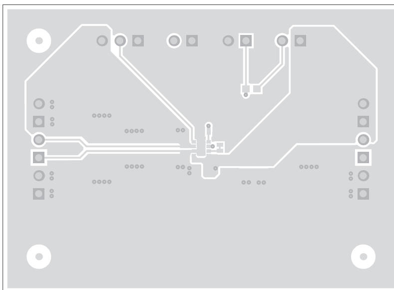
Figure 3. Top Layer
