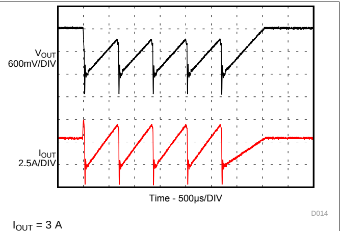
Figure 25. Short Circuit, HICUP Protection Entry / Exit
