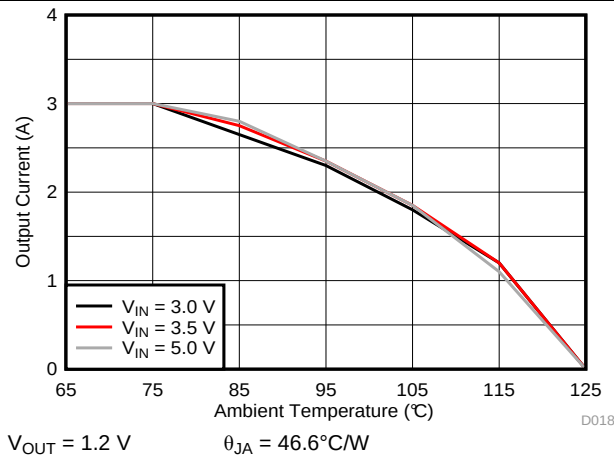
Figure 14. Thermal Derating
