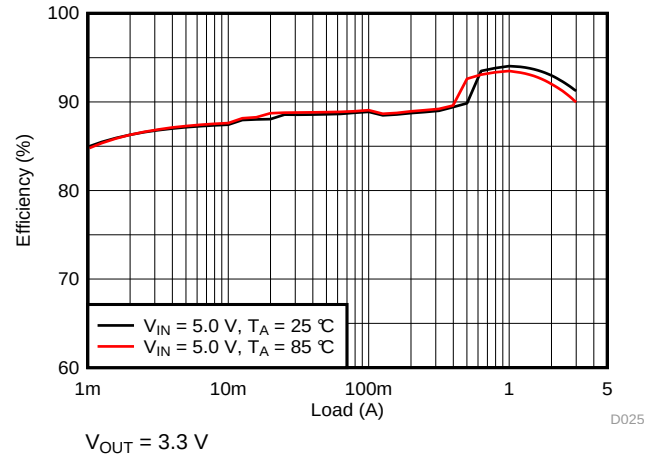
Figure 13. Efficiency
