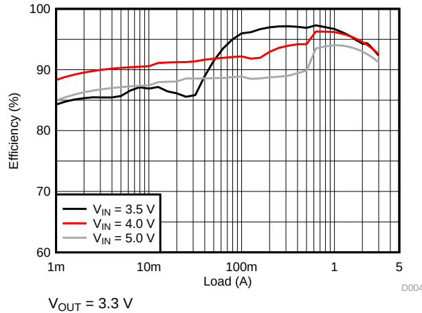
Figure 12. Efficiency
