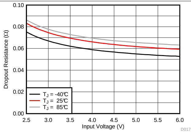
Figure 1. Dropout Resistance
