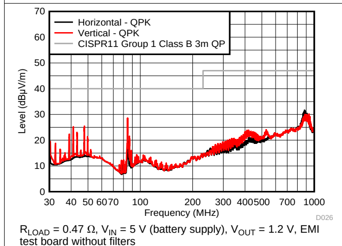
Figure 28. TPS82085 Radiated Emission
