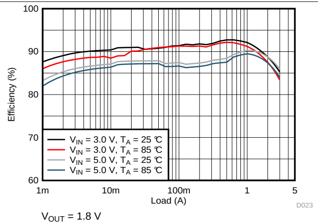
Figure 9. Efficiency
