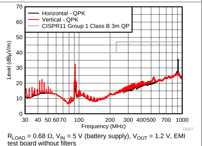
Figure 29. TPS82084 Radiated Emission
