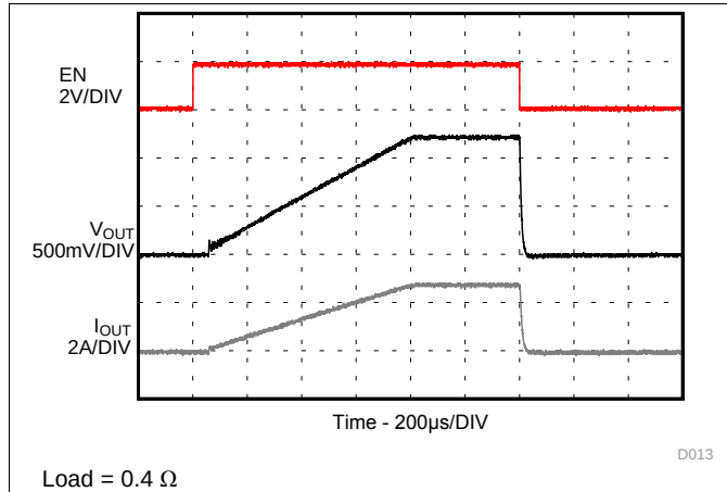
Figure 24. Startup / Shutdown with Resistive Load
