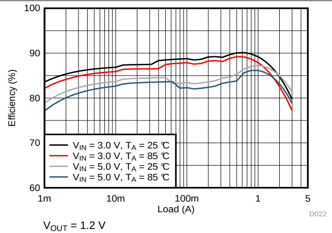
Figure 7. Efficiency
