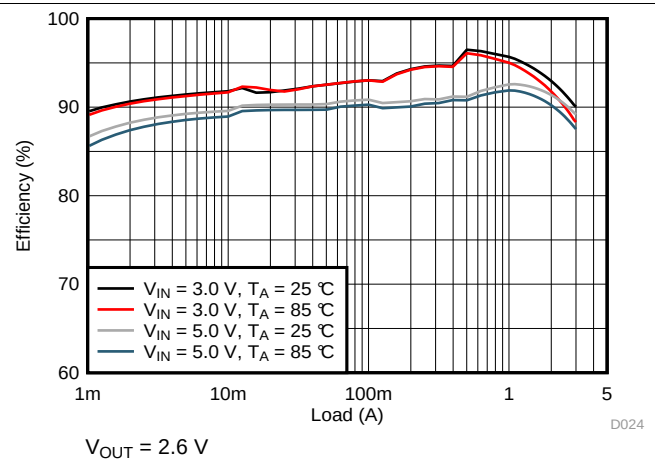
Figure 11. Efficiency
