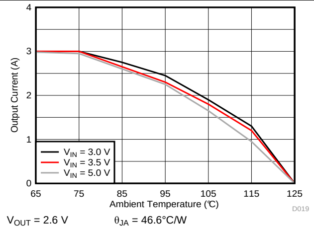
Figure 15. Thermal Derating
