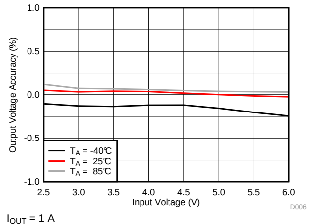
Figure 17. Line Regulation
