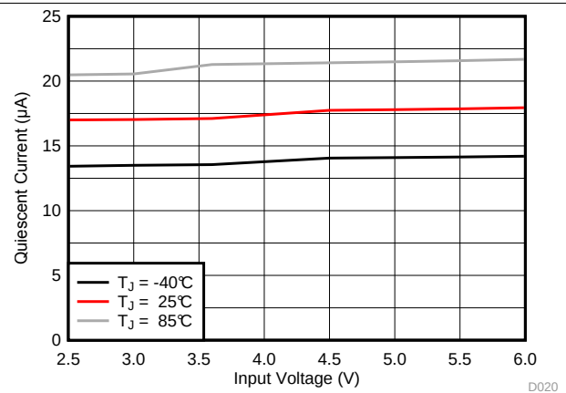
Figure 2. Quiescent Current
