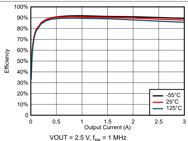
Figure 6-30. Efficiency for V_{\text{IN}} = 3.3\ \text{V}
