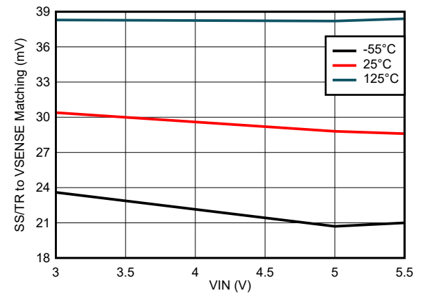
Figure 6-10. SS/TR to VSENSE Matching Variation
