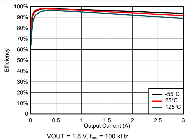
Figure 6-18. Efficiency for VIN = 3 V
