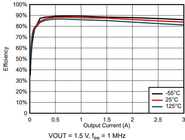
Figure 6-25. Efficiency for V_{\text{IN}} = 3\ \text{V}
