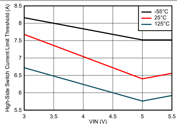
Figure 6-11. High-Side Switch Current Limit Threshold Variation
