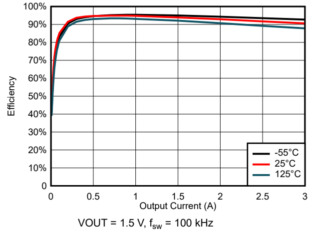
Figure 6-32. Efficiency for V_{\text{IN}} = 5\ \text{V}
