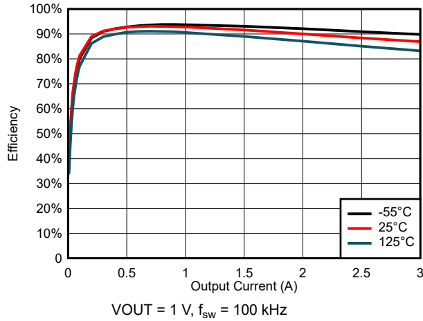
Figure 6-31. Efficiency for V_{\text{IN}} = 5\ \text{V}
