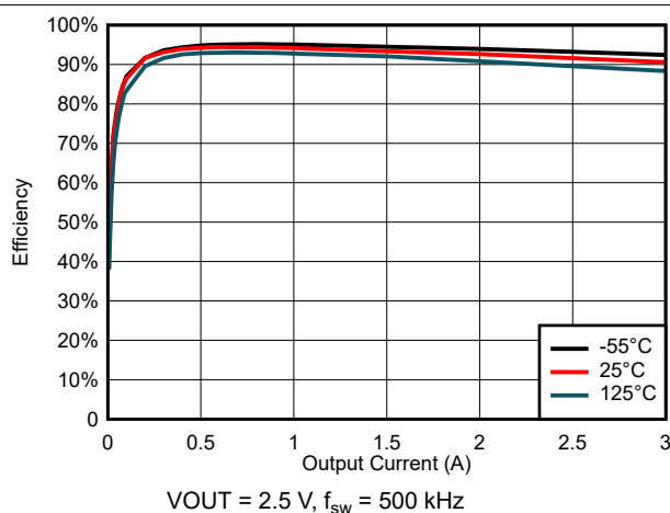
Figure 6-29. Efficiency for V_{\text{IN}} = 3.3\ \text{V}
