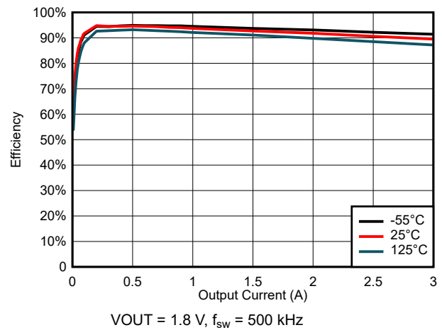
Figure 6-22. Efficiency for V_{\text{IN}} = 3\ \text{V}
