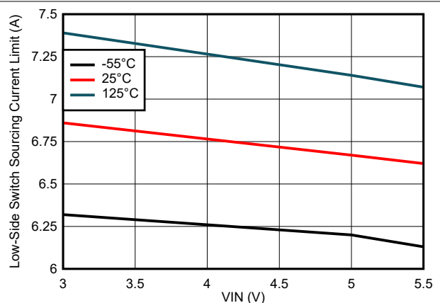
Figure 6-12. Low-Side Switch Sourcing Current Limit Variation
