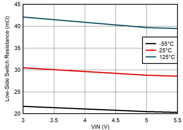
Figure 6-14. Low-Side Switch Resistance Variation
