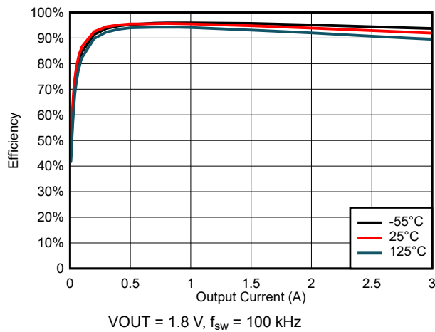
Figure 6-33. Efficiency for V_{\text{IN}} = 5\ \text{V}
