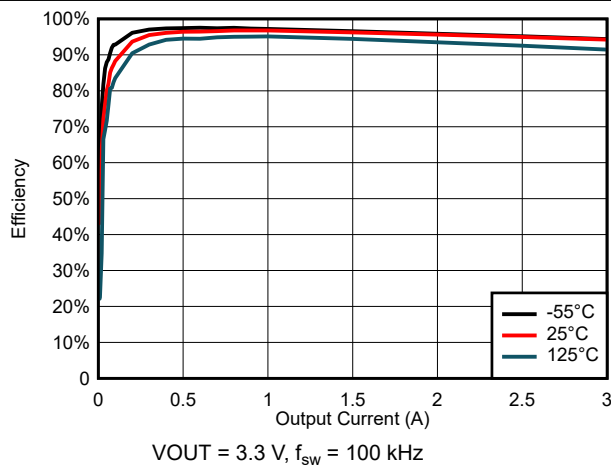
Figure 6-35. Efficiency for V_{\text{IN}} = 5\ \text{V}
