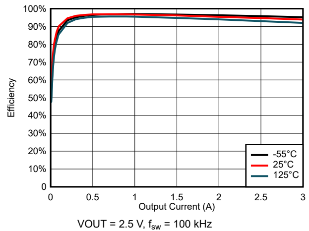
Figure 6-34. Efficiency for V_{\text{IN}} = 5\ \text{V}
