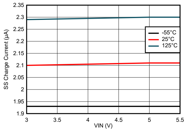
Figure 6-9. SS Charge Current Variation
