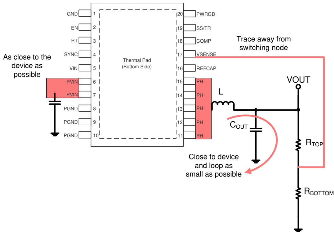
Figure 10-1. PCB Layout Example
