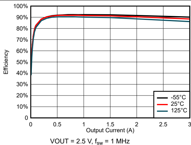
Figure 6-27. Efficiency for V_{\text{IN}} = 3\ \text{V}
