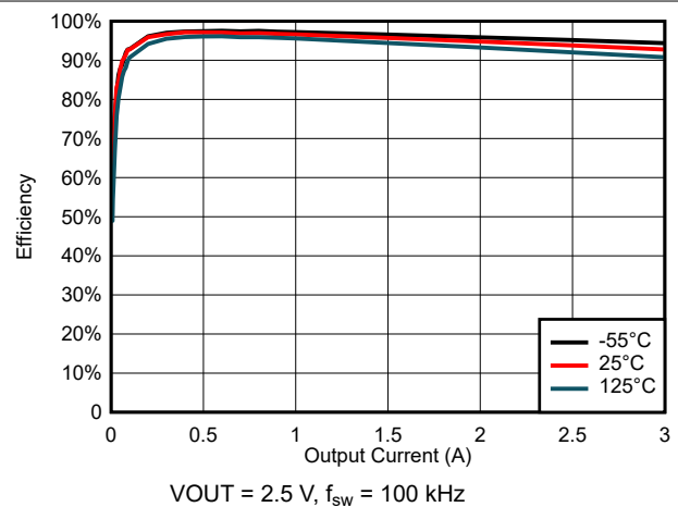
Figure 6-28. Efficiency for V_{\text{IN}} = 3.3\ \text{V}
