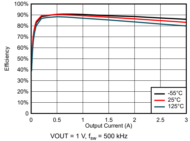
Figure 6-20. Efficiency for V_{\text{IN}} = 3\ \text{V}
