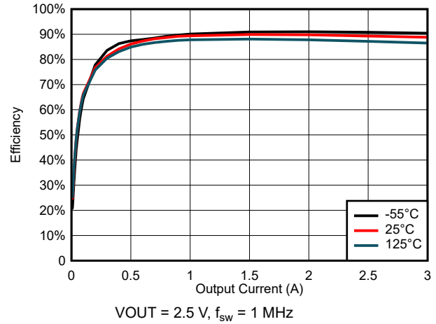
Figure 6-56. Efficiency for V_{\text{IN}} = 5.5\ \text{V}
