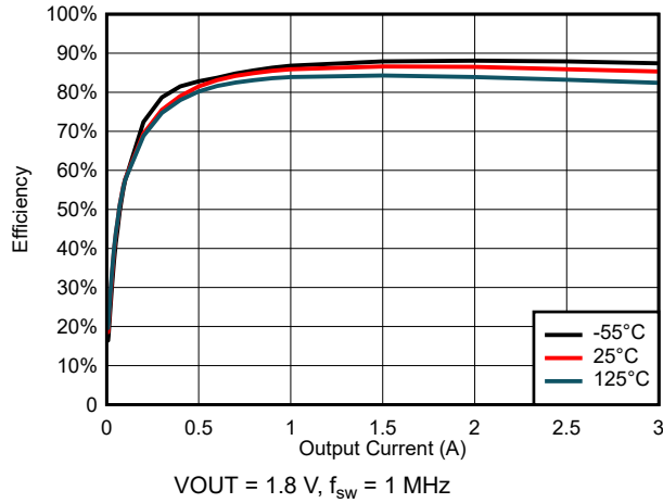
Figure 6-55. Efficiency for V_{\text{IN}} = 5.5\ \text{V}
