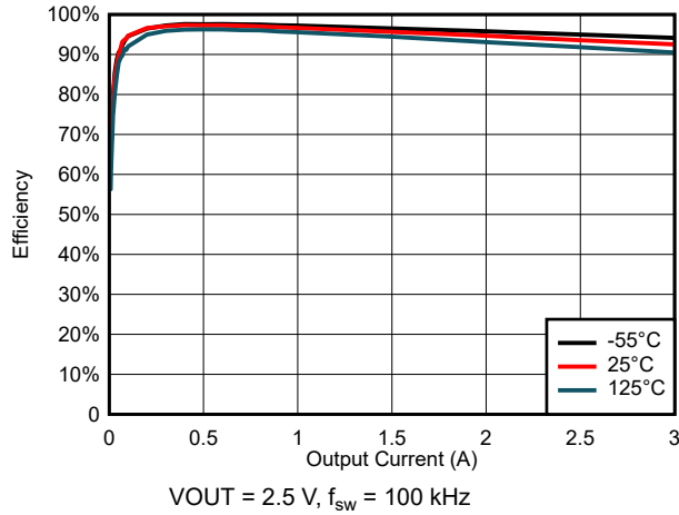
Figure 6-19. Efficiency for V_{\text{IN}} = 3\ \text{V}
