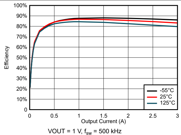
Figure 6-36. Efficiency for V_{\text{IN}} = 5\ \text{V}
