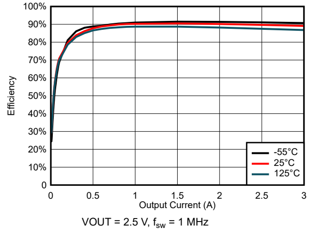
Figure 6-44. Efficiency for V_{\text{IN}} = 5\ \text{V}
