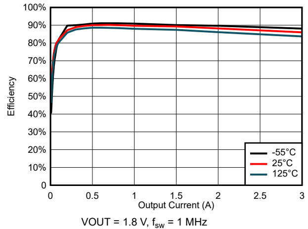
Figure 6-26. Efficiency for V_{\text{IN}} = 3\ \text{V}
