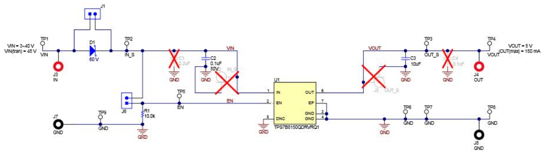
Figure 4. TPS7B81EVM-025 Schematic
