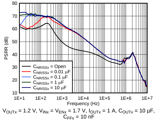
Figure 2. Power-Supply Rejection vs C_{\text{NR/SSX}}
