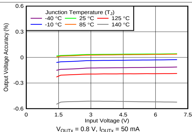
Figure 26. Line Regulation
