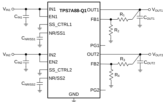
Figure 45. Adjustable Operation
