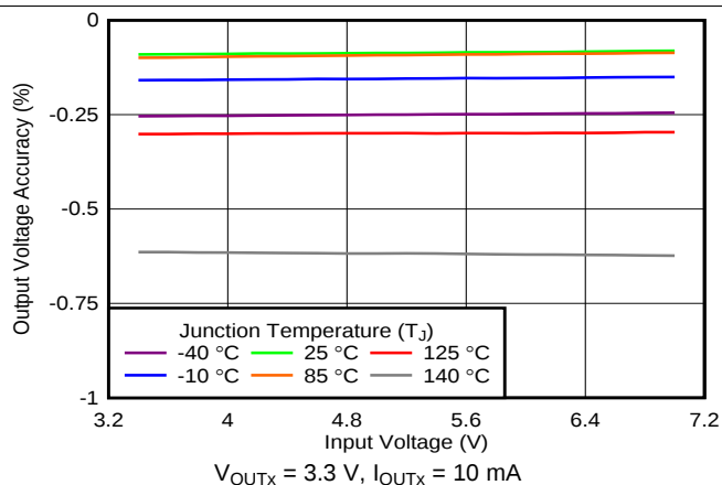
Figure 28. Line Regulation
