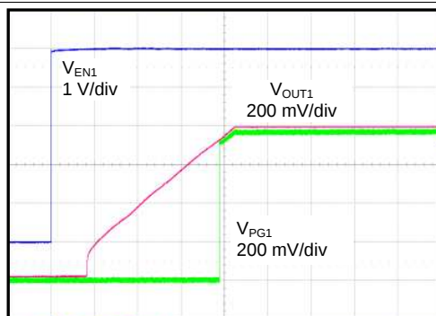
Figure 19. Start-Up
