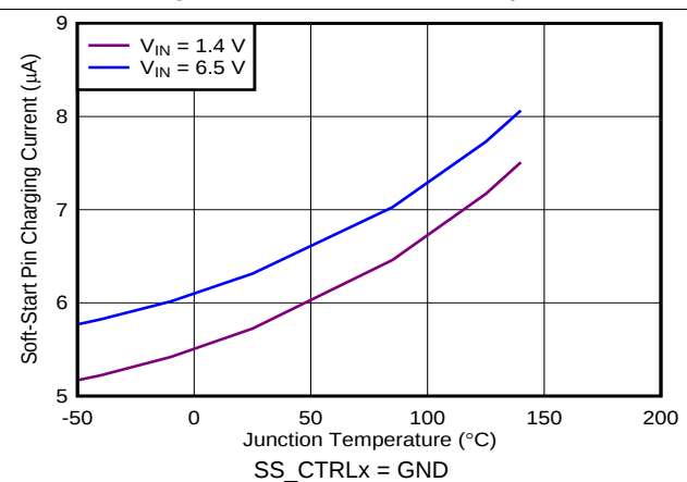
Figure 36. Soft-Start Current vs Temperature
