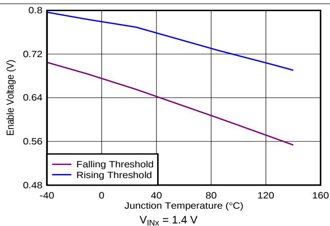
Figure 38. Enable Threshold vs Temperature
