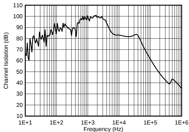
Figure 57. Channel-to-Channel Isolation
