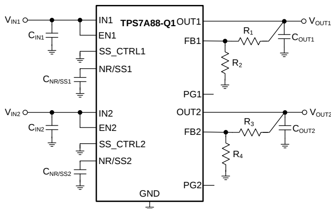
Figure 55. Application Example
