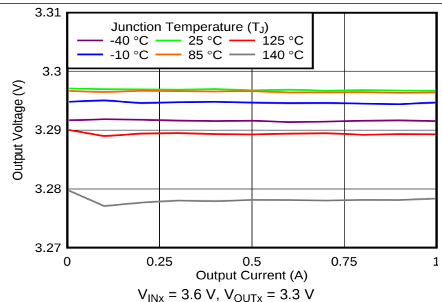
Figure 27. Load Regulation
