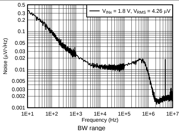
Figure 58. Output Noise
