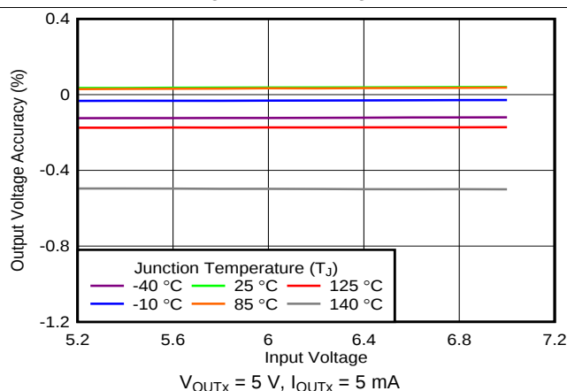
Figure 30. Line Regulation
