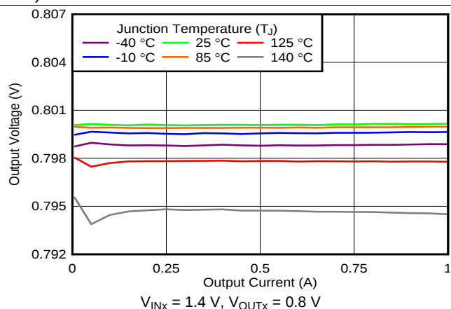
Figure 25. Load Regulation
