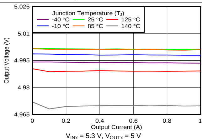
Figure 29. Load Regulation
