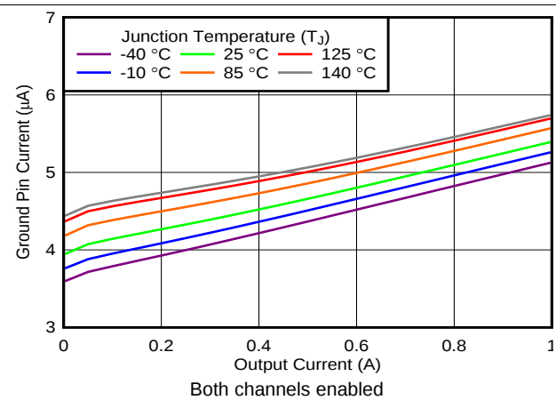
Figure 32. Ground Current vs Output Current
