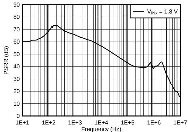
Figure 56. Power-Supply Rejection
