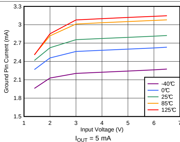
Figure 35. Ground Pin Current vs Input Voltage
