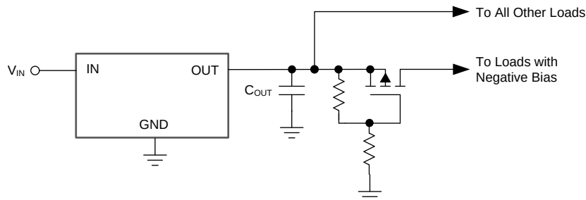
Figure 56. PMOSFET to Isolate the Output from the Load
