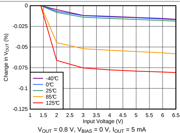
Figure 29. Line Regulation without Bias
