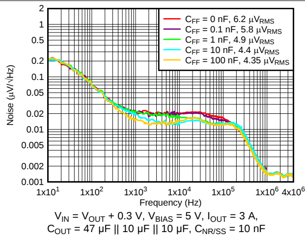
Figure 13. Output Noise vs Frequency and C_{FF}
