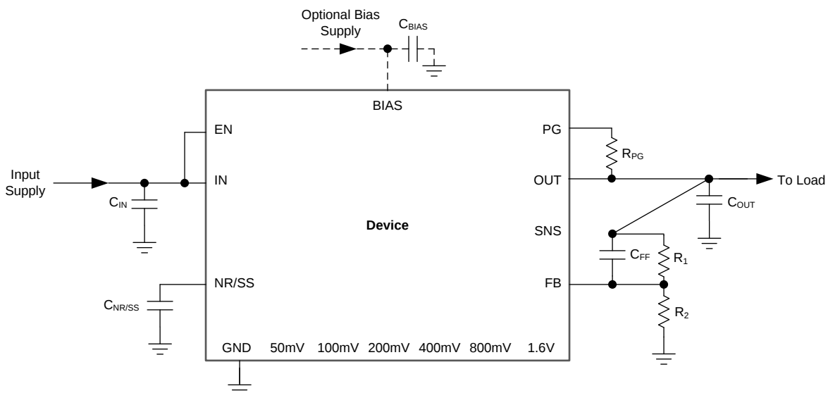
Figure 54. Typical Application
