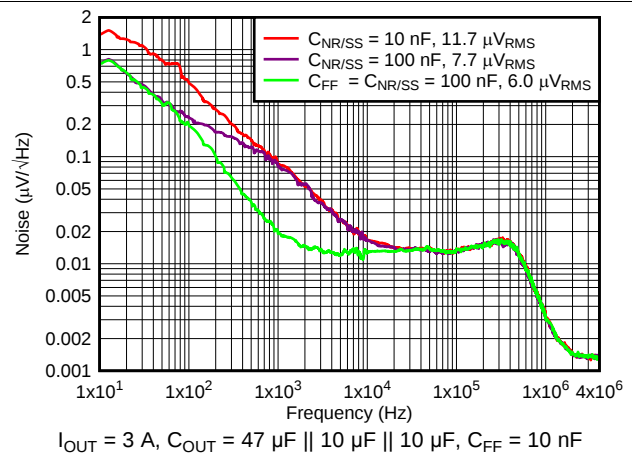
Figure 14. Output Noise at 5.0-V Output
