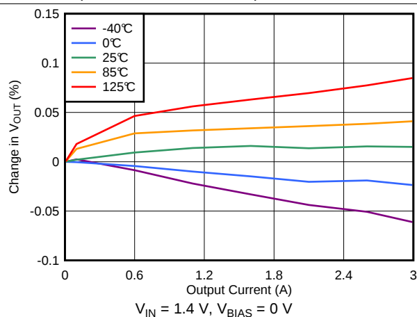
Figure 26. Load Regulation with Bias
