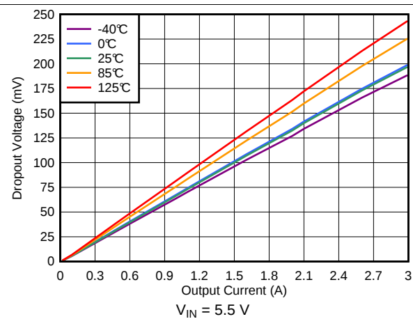
Figure 24. Dropout Voltage vs Output Current (High V_{IN} )
