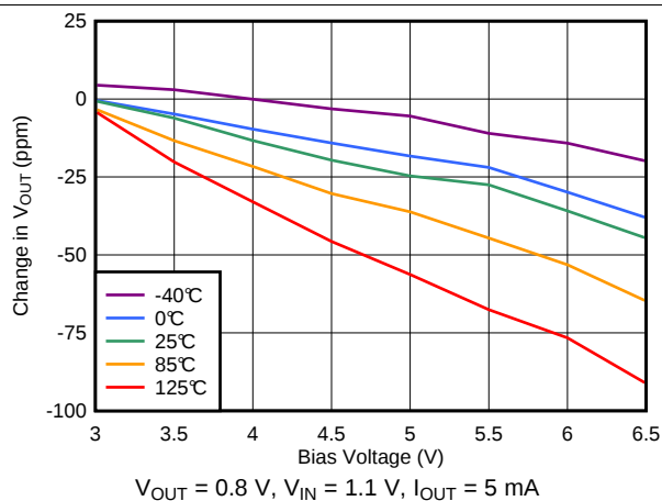
Figure 30. Line Regulation without Bias
