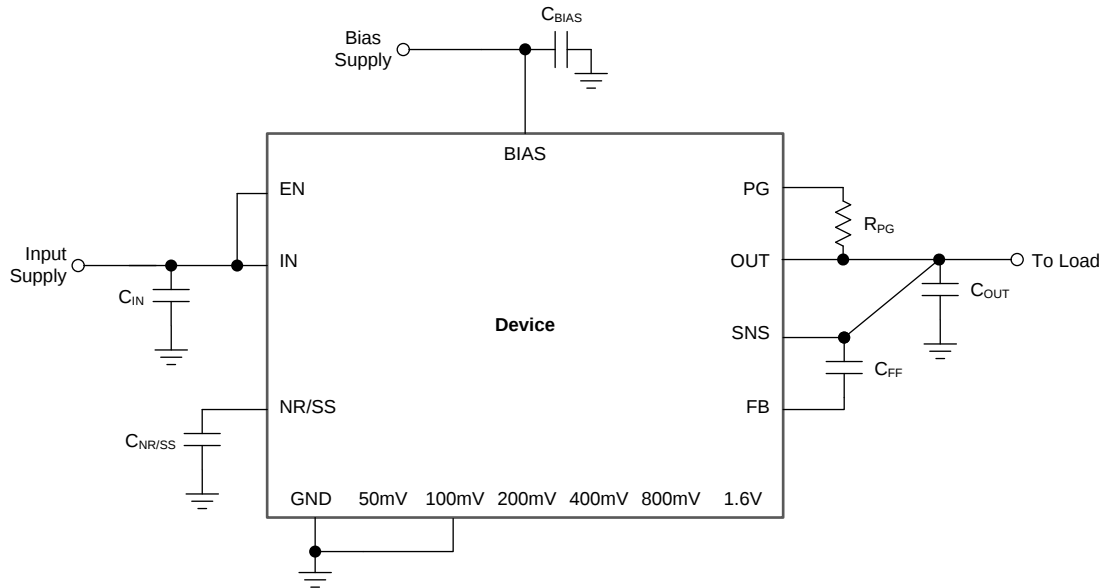
Figure 51. Typical Application
