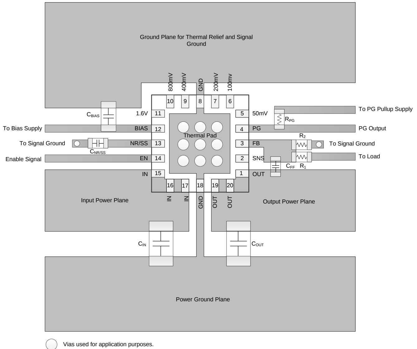
Figure 57. Example Layout
