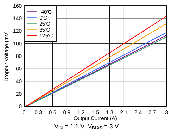
Figure 23. Dropout Voltage vs Output Current with Bias
