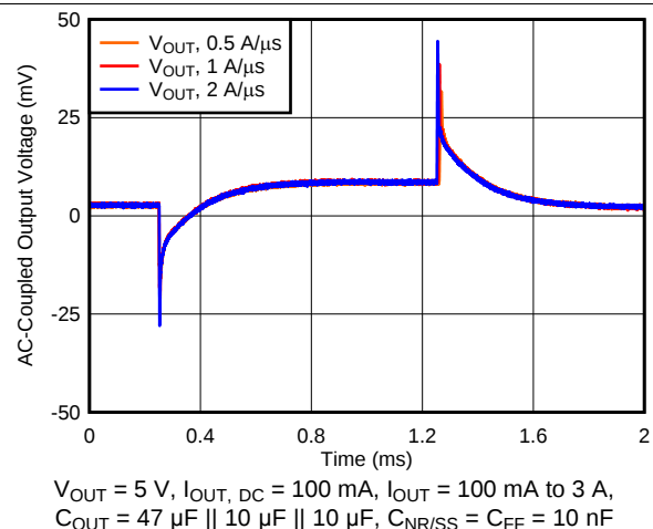
Figure 18. Load Transient vs Time and Slew Rate
