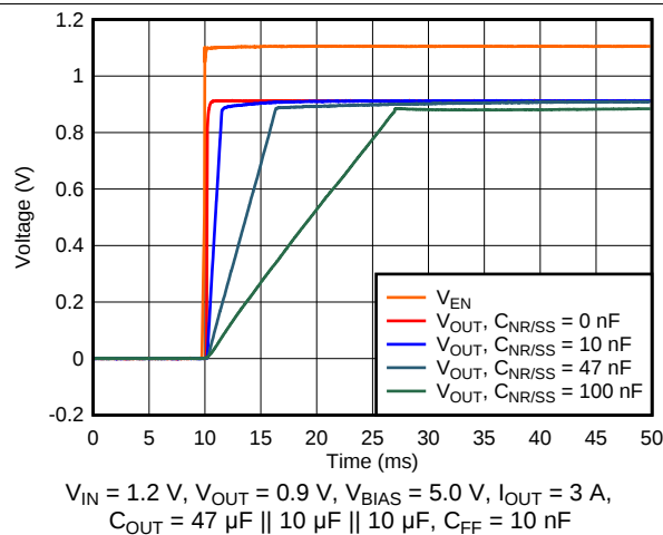
Figure 15. Start-Up Waveform vs Time and C_{NR/SS}
