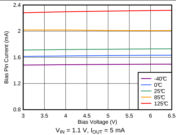
Figure 33. Quiescent Current vs Bias Voltage
