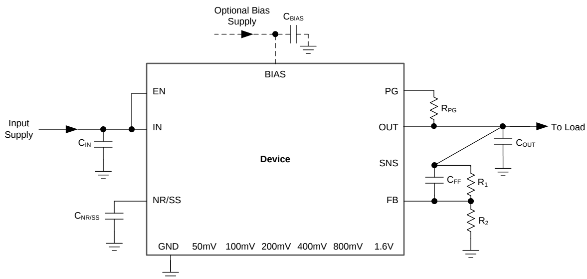
Figure 45. Adjustable Operation
