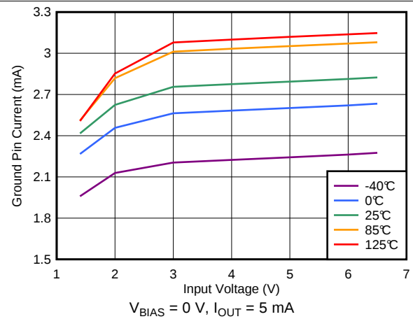
Figure 32. Quiescent Current vs Input Voltage
