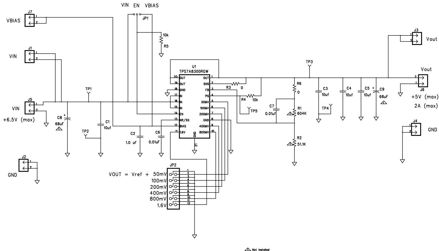
Figure 4. TPS7A8300EVM-209 Schematic
