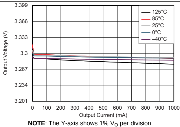
Figure 1. Load Regulation
