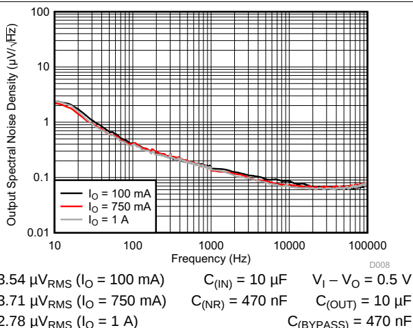
Figure 36. Output Spectral Noise Density vs Frequency (RMS noise (100 Hz to 100 kHz))
