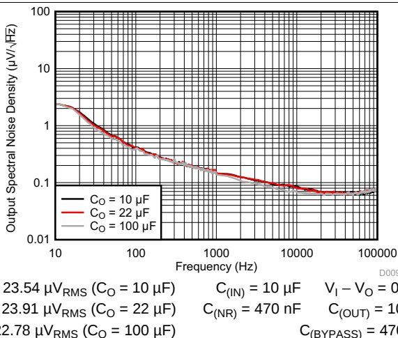
Figure 24. Output Spectral Noise Density vs Frequency (RMS noise (100 Hz to 100 kHz))
