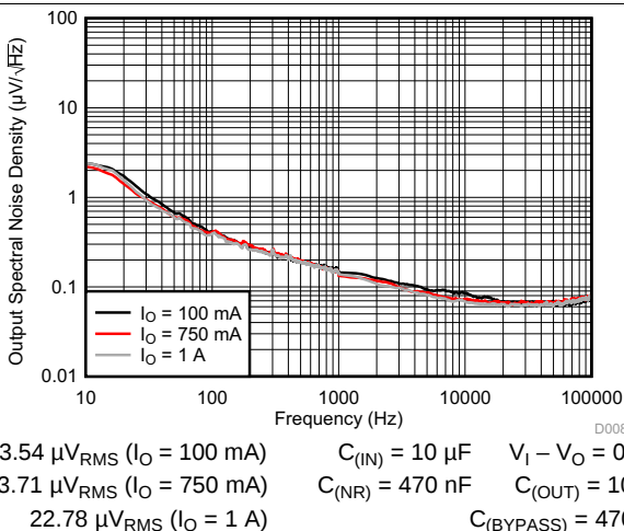
Figure 23. Output Spectral Noise Density vs Frequency (RMS noise (100 Hz to 100 kHz))
