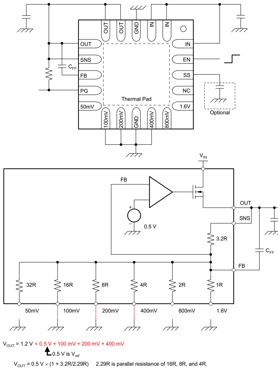
Figure 23. 1.2-V Configuration
