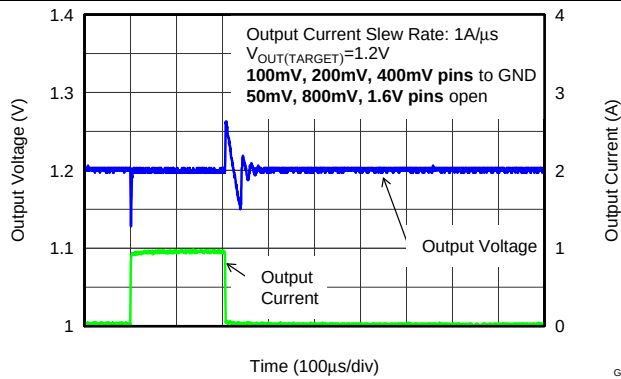
Figure 30. Load Transient Response (V OUT = 1.2 V)
