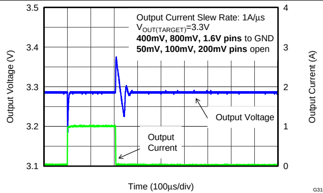
Figure 31. Load Transient Response (V OUT = 3.3 V)
