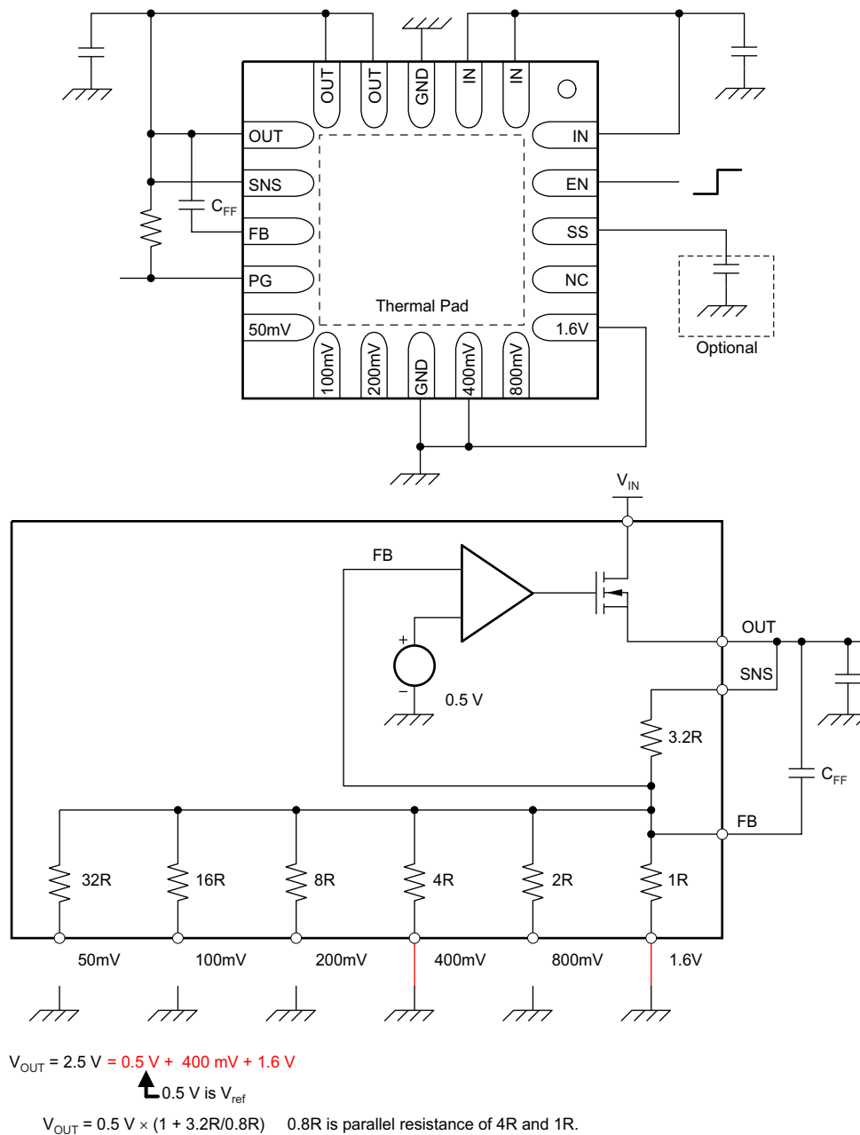
Figure 25. 2.5-V Configuration
