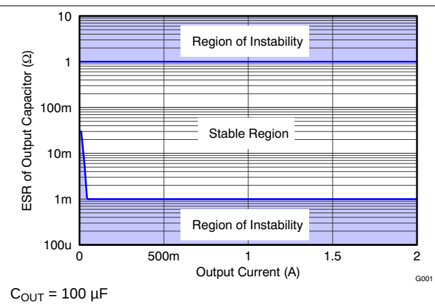
Figure 2. Stability Curve
