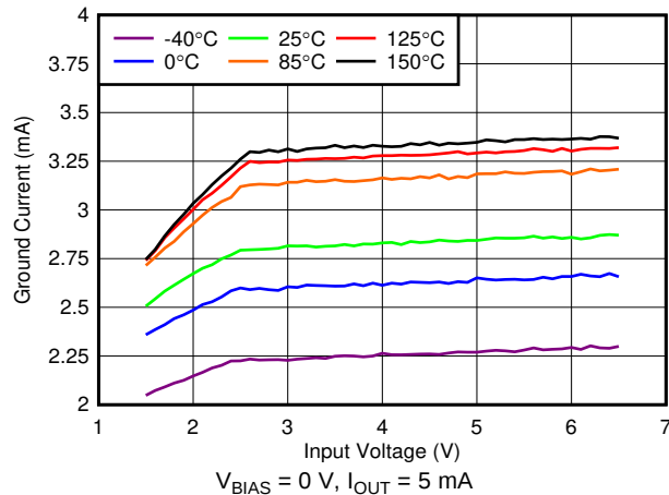
Figure 27. Ground Current vs Input Voltage
