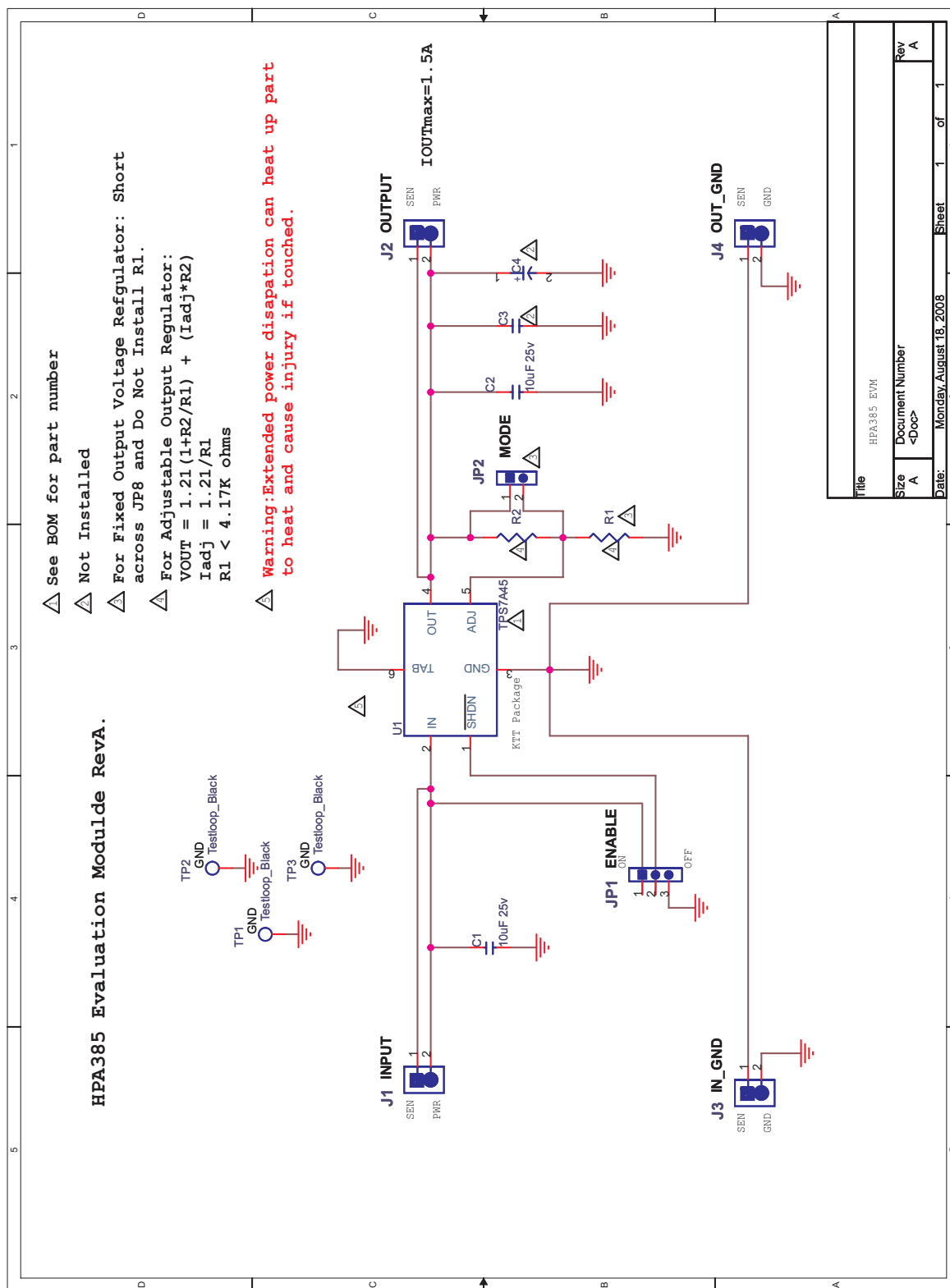
Figure 9. EVM Schematic
