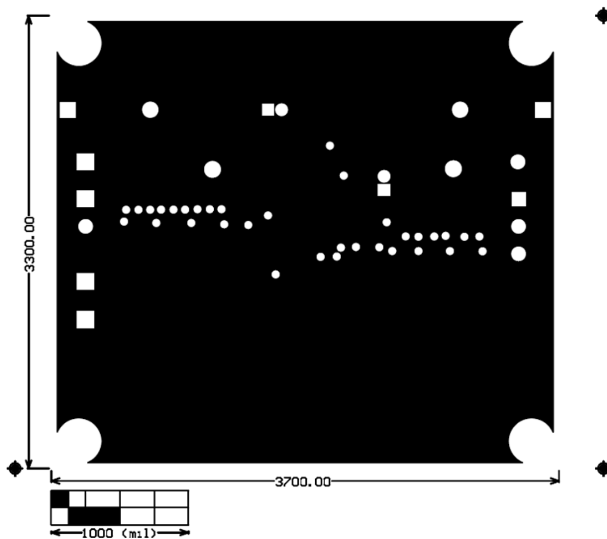
Figure 3. Board Layout - Second Layer (Mid Layer 1) Ground Plane
