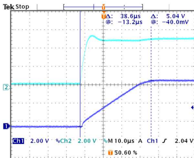
Figure 12. V_{OUT} and V_{IN} With no Soft-Start
