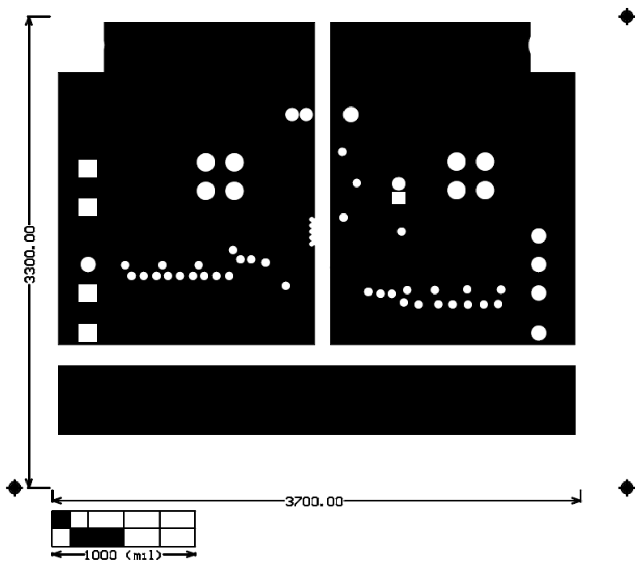
Figure 4. Board Layout - Third Layer (Mid Layer 2) Power Plane
