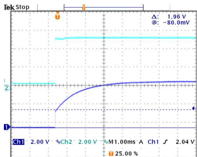
Figure 13. V_{OUT} and V_{IN} With Soft-Start Circuit
