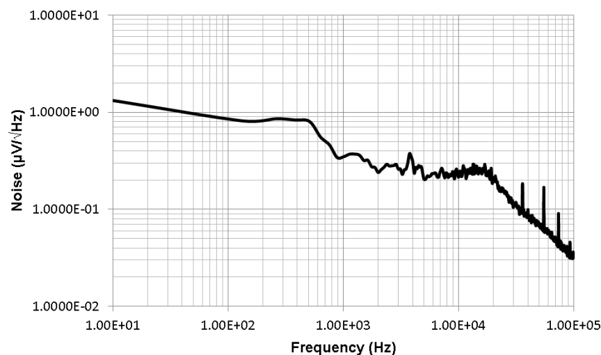
Figure 15. Worst-Case RMS Noise (10 Hz - 100 kHz) = 47.39 \mu V_{rms} , V_{IN} = 5.5 V, V_{OUT} = 5 V at 1.5 A Load
