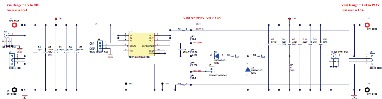
Figure 17. TPS7A4501SPEVM Schematic
