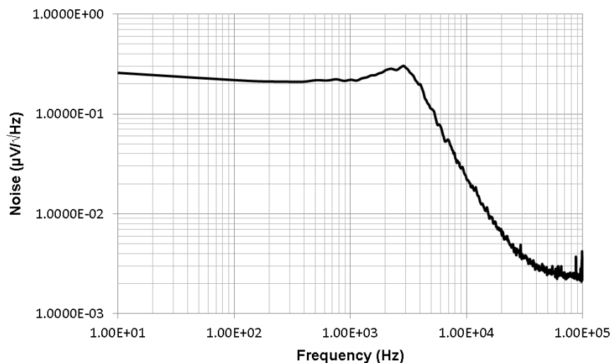
Figure 14. Best-Case RMS Noise (10 Hz - 100 kHz) = 16.86 \mu V_{rms} , V_{IN} = 5.5 V, V_{OUT} = 5 V at no Load
