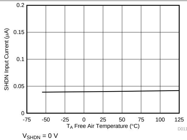
Figure 9. SHDN Input Current vs Temperature
