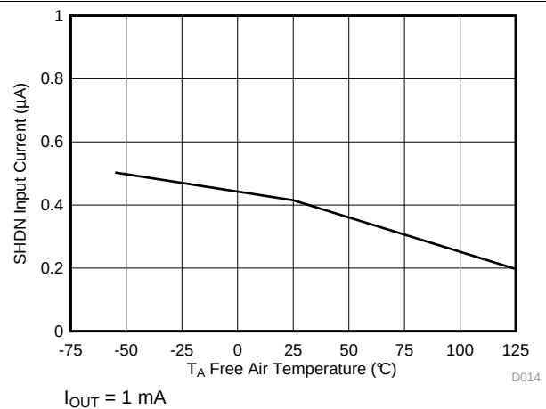
Figure 12. SHDN Threshold (On to Off) vs Temperature
