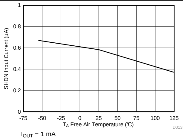
Figure 11. SHDN Threshold (Off To On) vs Temperature
