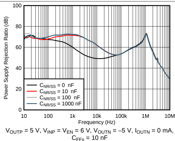
Figure 10. Positive PSRR vs Frequency and C_{\text{NR/SS}}
