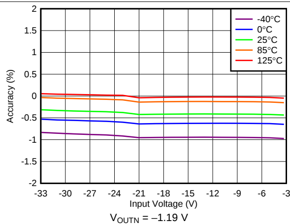
Figure 34. Negative Line Regulation
