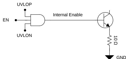
Figure 62. Simplified Active Discharge Circuit
