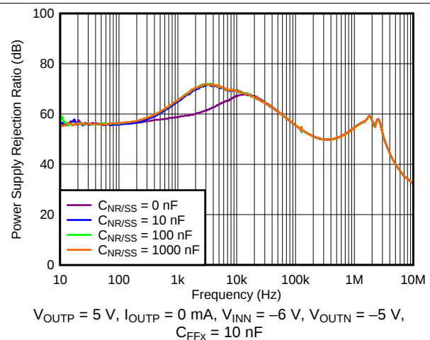
Figure 11. Negative PSRR vs Frequency and C_{\text{NR/SS}}
