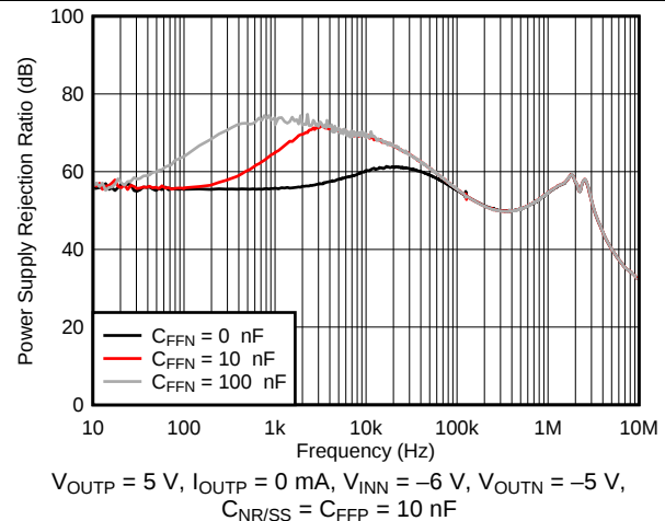
Figure 9. Negative PSRR vs Frequency and C_{\text{FFN}}
