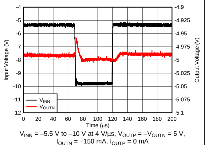
Figure 29. Line Transient Negative Regulator
