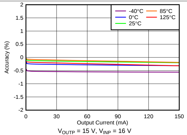
Figure 41. Positive Load Regulation
