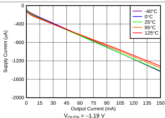
Figure 57. Negative Supply Current vs Output Current
