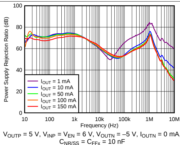
Figure 4. Positive PSRR vs Frequency and I_{OUTP}
