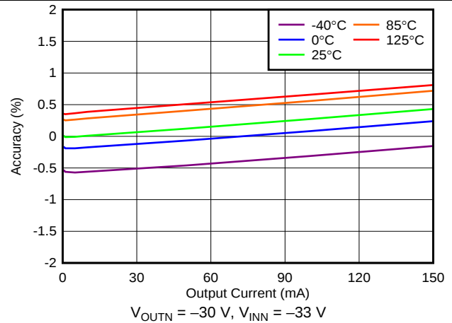
Figure 39. Negative Load Regulation
