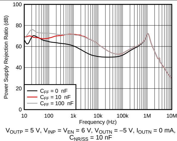
Figure 8. Positive PSRR vs Frequency and C_{\text{FFP}}
