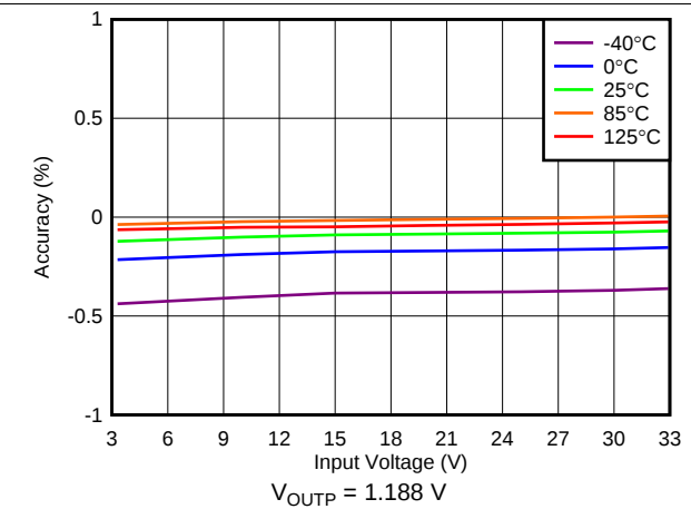
Figure 43. Positive Line Regulation
