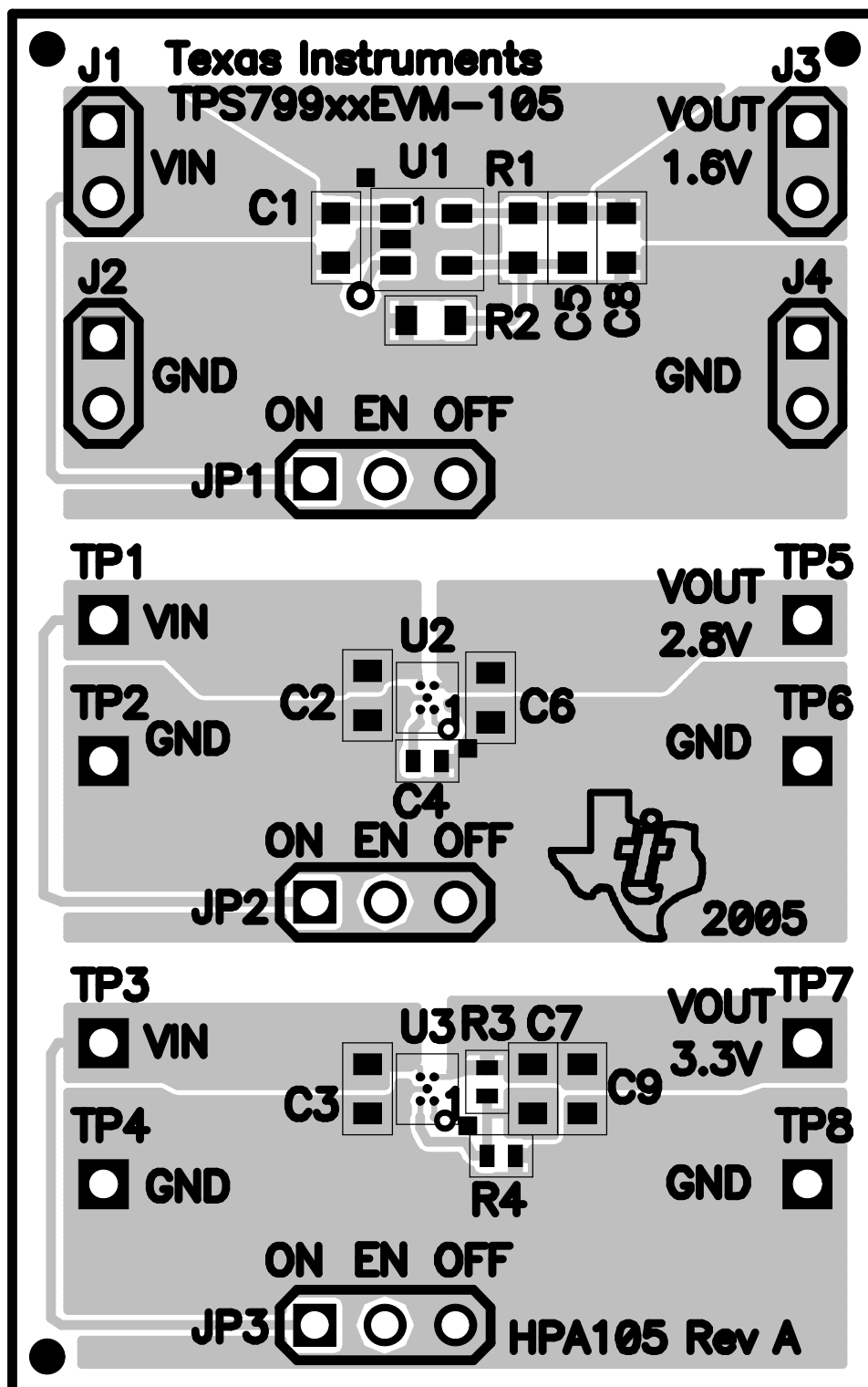
Figure 1. Assembly Layer
