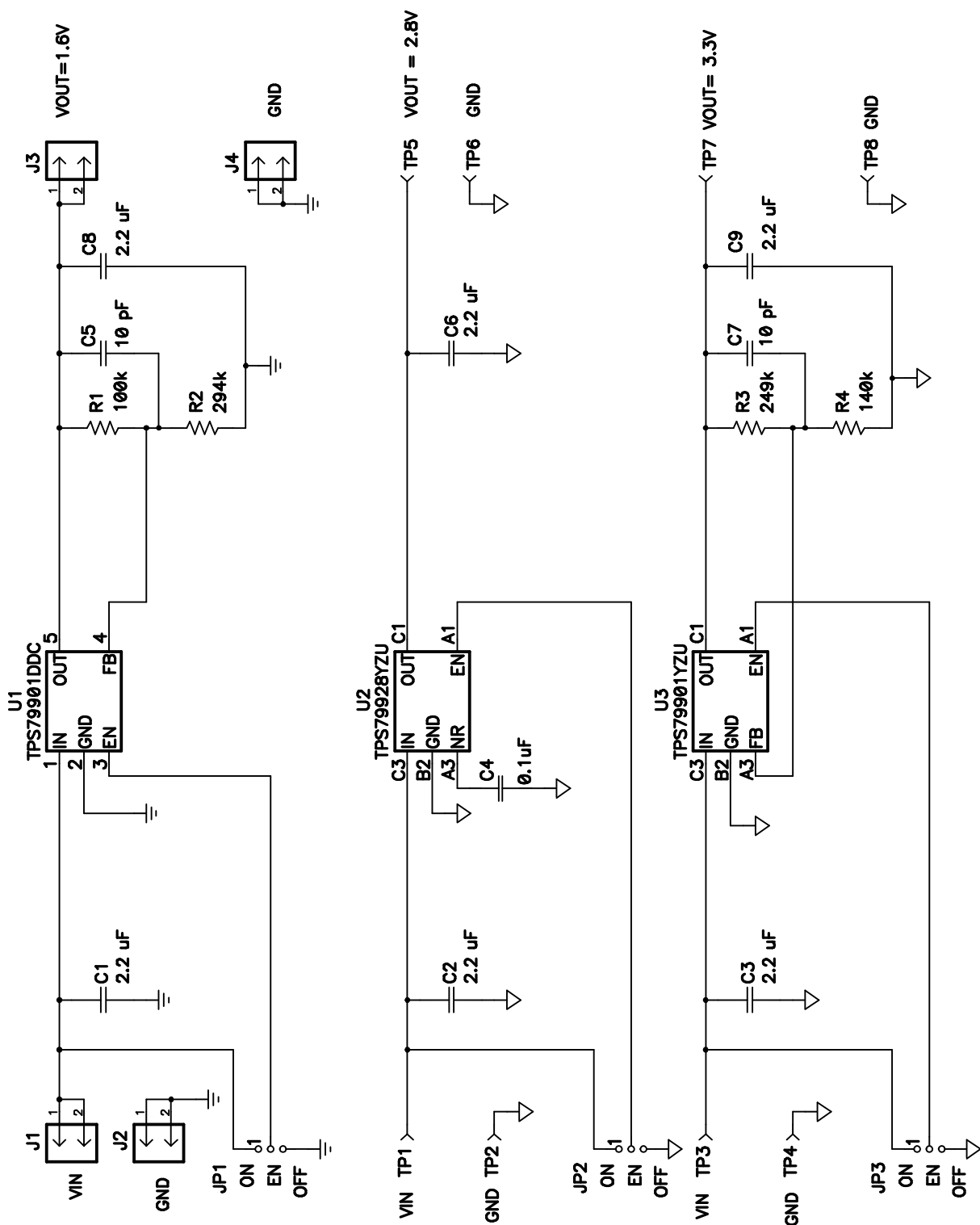
Figure 4. TPS799xxEVM-105 Schematic
