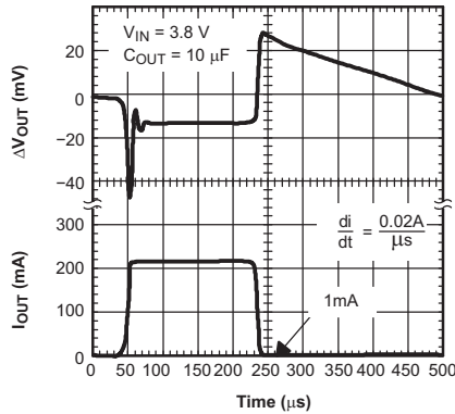
Figure 27. TPS79328 Load Transient Response
