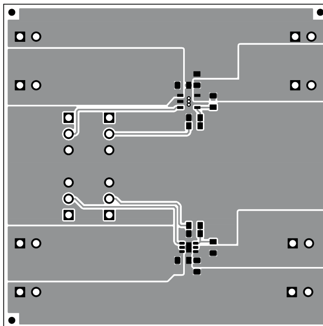
Figure 6. Top Layer
