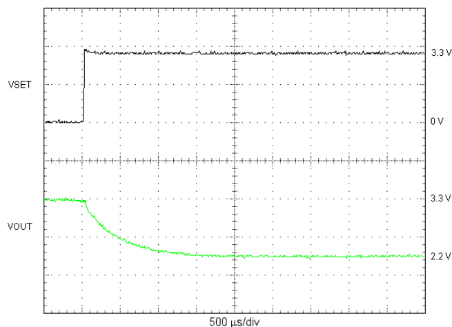
Figure 4. High to Low Output Transient, TPS781330220 ( V_{OUT} = 3.3 V to 2.2 V, R_{LOAD} = 22 \Omega )
