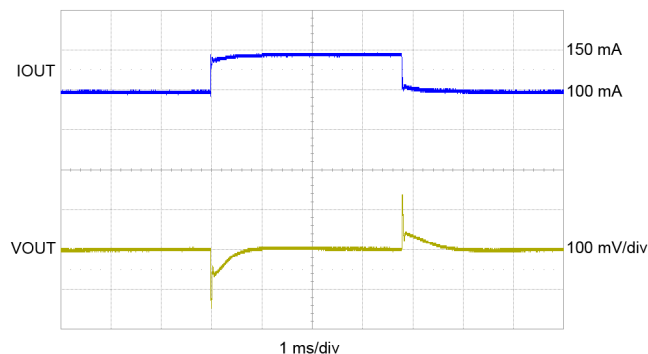
Figure 2. Load Transient, TPS78101, V_I = 3.6 V, V_{OUT} = 3.0 V, I_{OUT} = 100 mA to 150 mA to 100 mA
