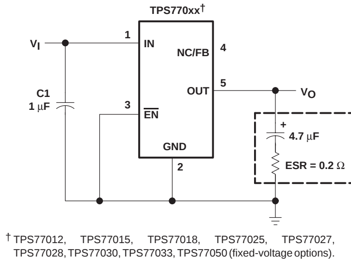
Figure 21. Typical Application Circuit
