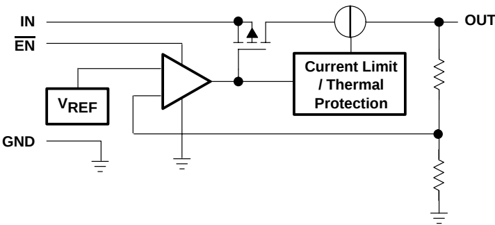
TPS76912/15/18/25/27/28/30/33/50
