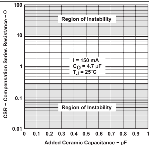
Figure 17. Compensation Series Resistance (CSR) vs Added Ceramic Capacitance
