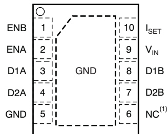
DSK Package 10-Pin WSON Top View
