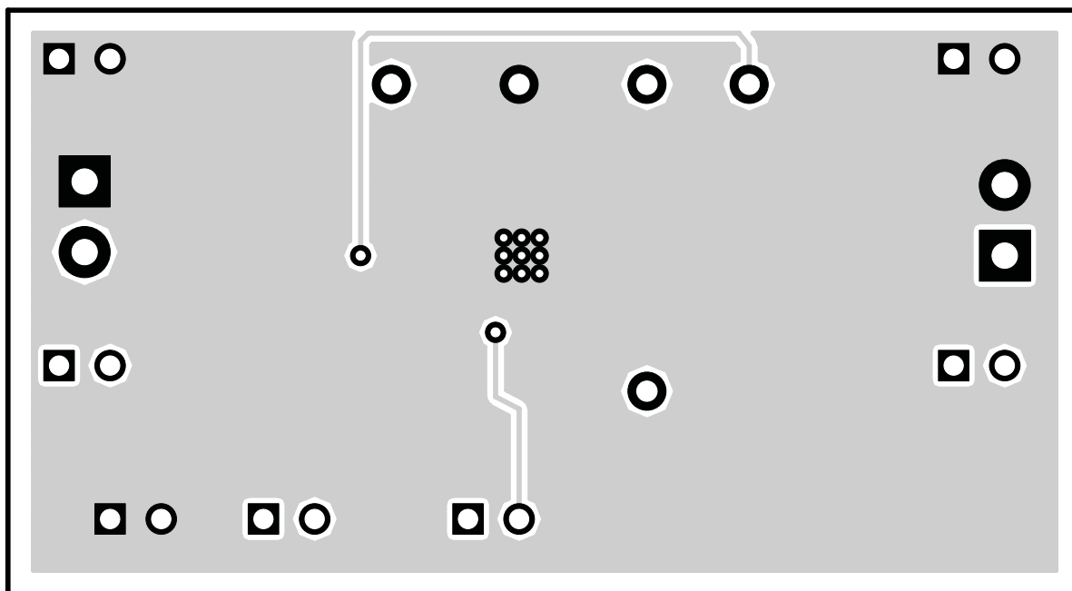
Figure 4. Bottom Layer
