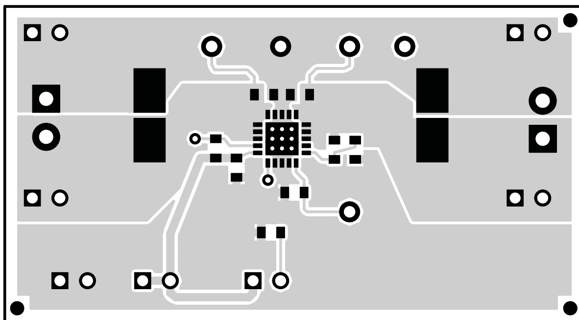
Figure 3. Top Layer
