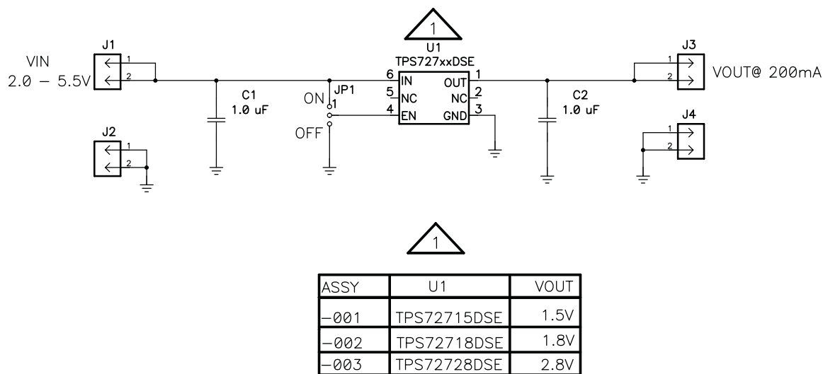
Figure 5. TPS727xxDSEEVm-406 Schematic
