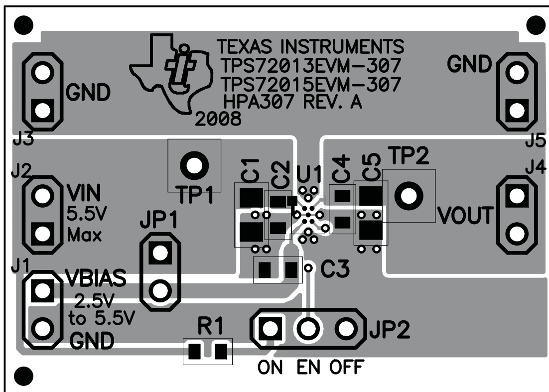
Figure 3. Top Assembly Layer
