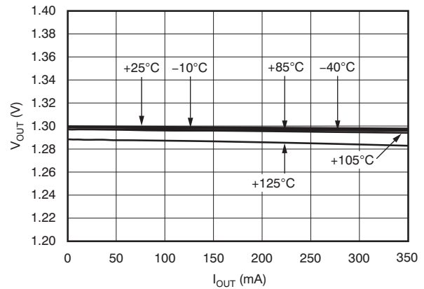
Figure 30. Load Regulation (TPS72013YZU)
