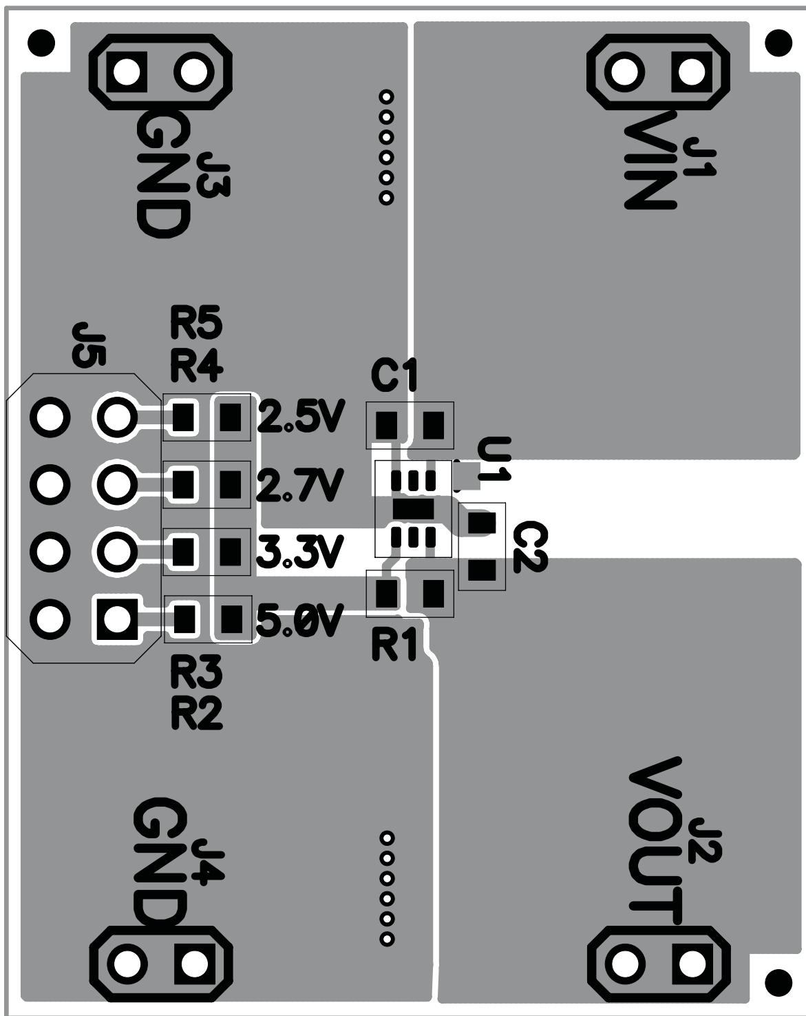
Figure 1. Assembly Layer
