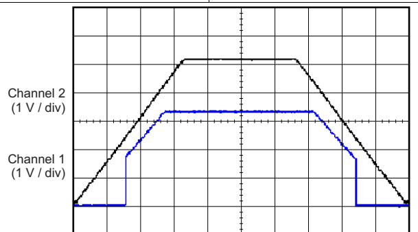
Figure 40. Power-Up and Power-Down Response
