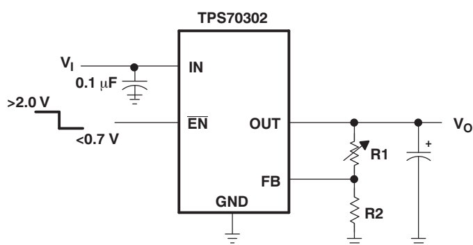
Figure 45. TPS70302 Adjustable LDO Regulator Programming
