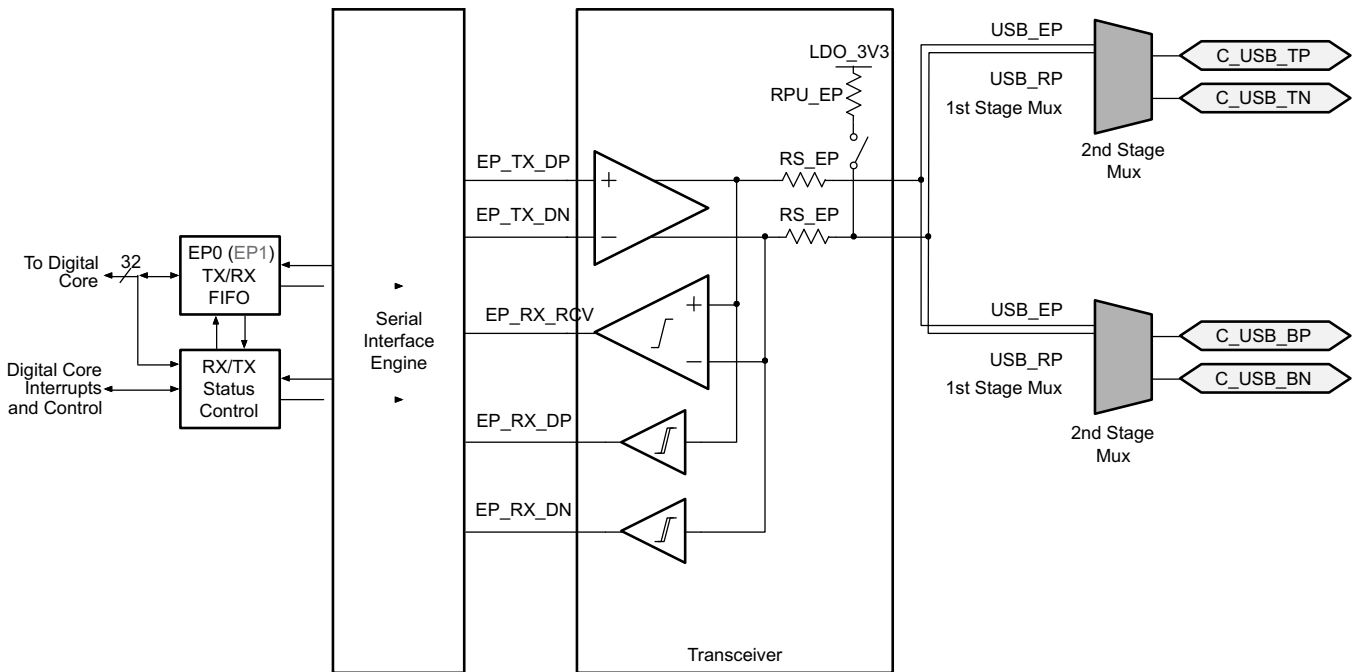
Figure 44. USB Endpoint Phy
