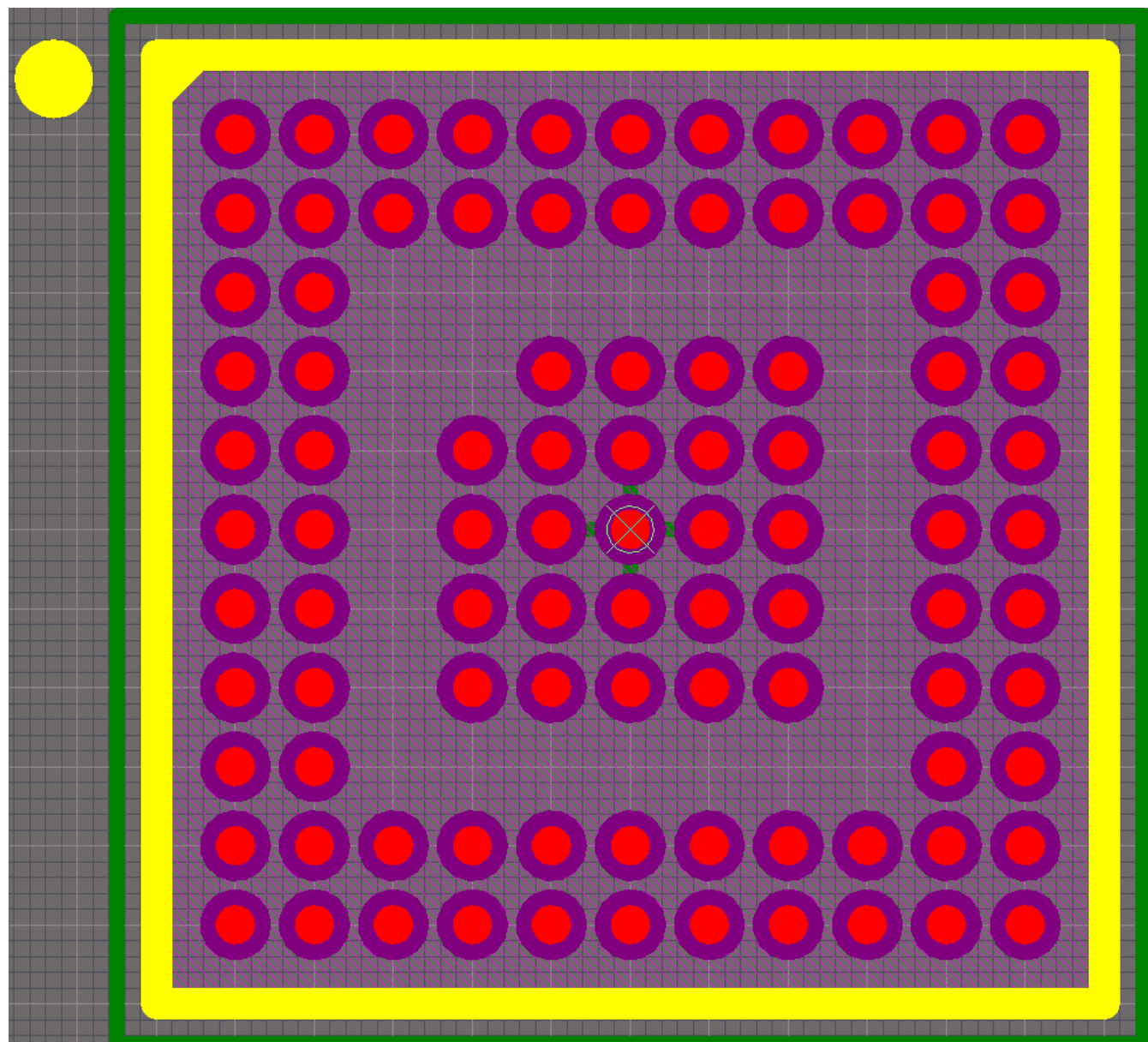
Figure 88. Top View Standard TPS65986 Footprint (Circular Pads)
