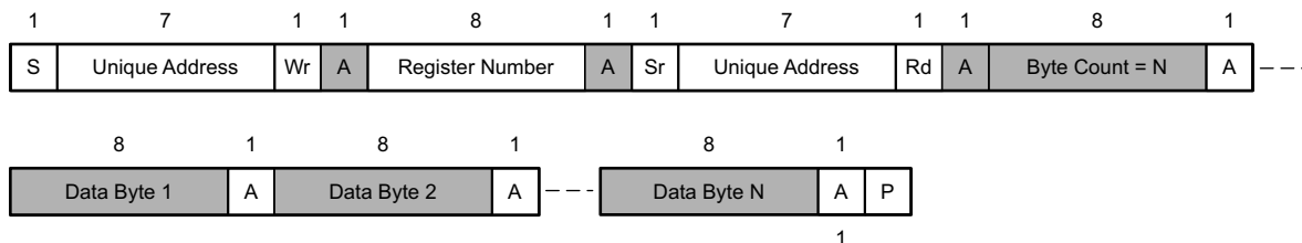
Figure 71. I²C Unique Address Read Register Protocol
