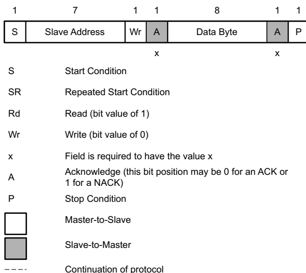
Figure 72. I²C Read/Write Protocol Key
