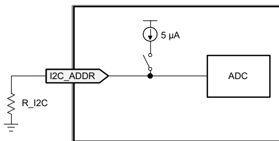
Figure 73. I²C Address Decode
