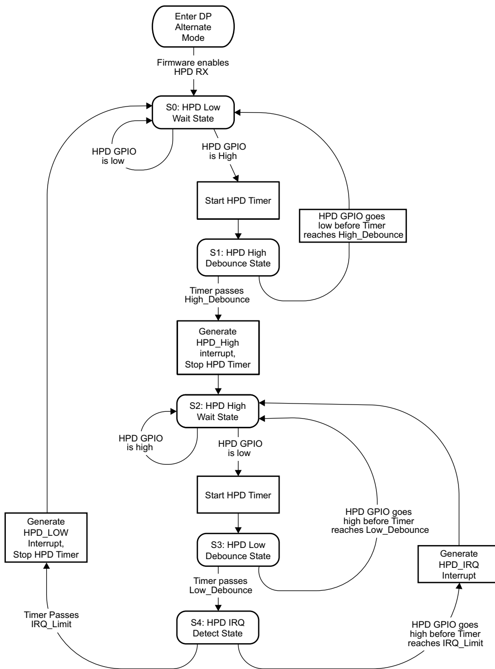
Figure 49. HPD TX Flow Diagram
