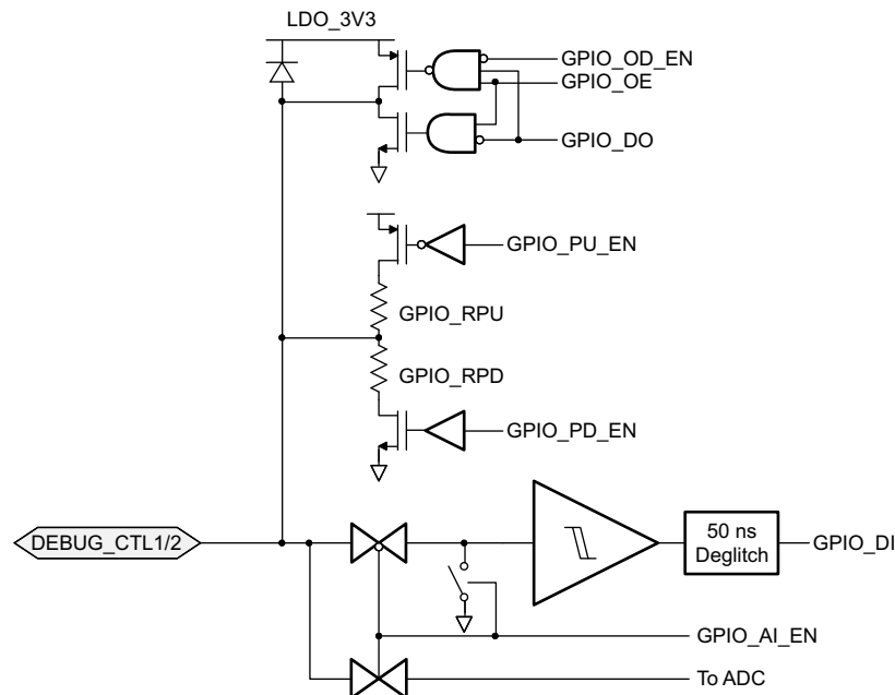
Figure 52. IOBUF_GPIOLSI2C (General GPIO) I/O with I²C De-glitch
