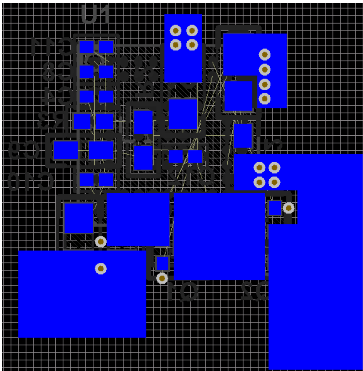
Figure 98. Bottom Polygonal Pours
