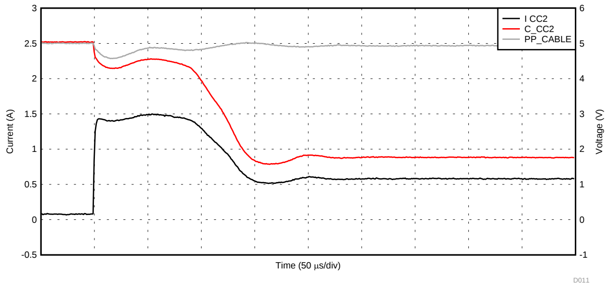
Figure 39. PP_CABLE to C_CCn Current Limit Response with a Soft Short (2 Ω)
