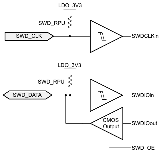
Figure 59. IOBUF_GPIOHSSWD
