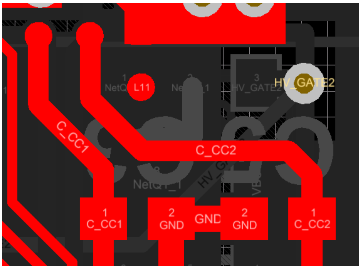
Figure 99. CC1 and CC2 Capacitor Routing
