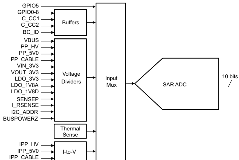
Figure 50. SAR ADC
