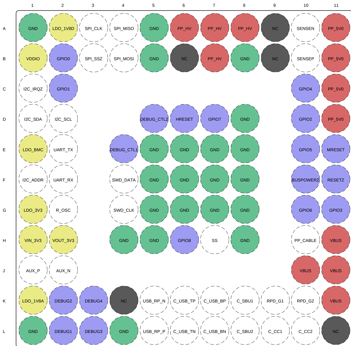
ZQZ Package 96-Pin BGA Top View
