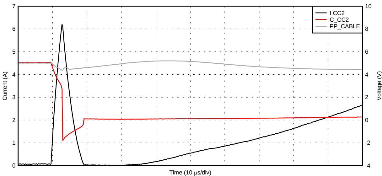
Figure 37. PP_CABLE to C_CCn Current Limit with a Hard Short
