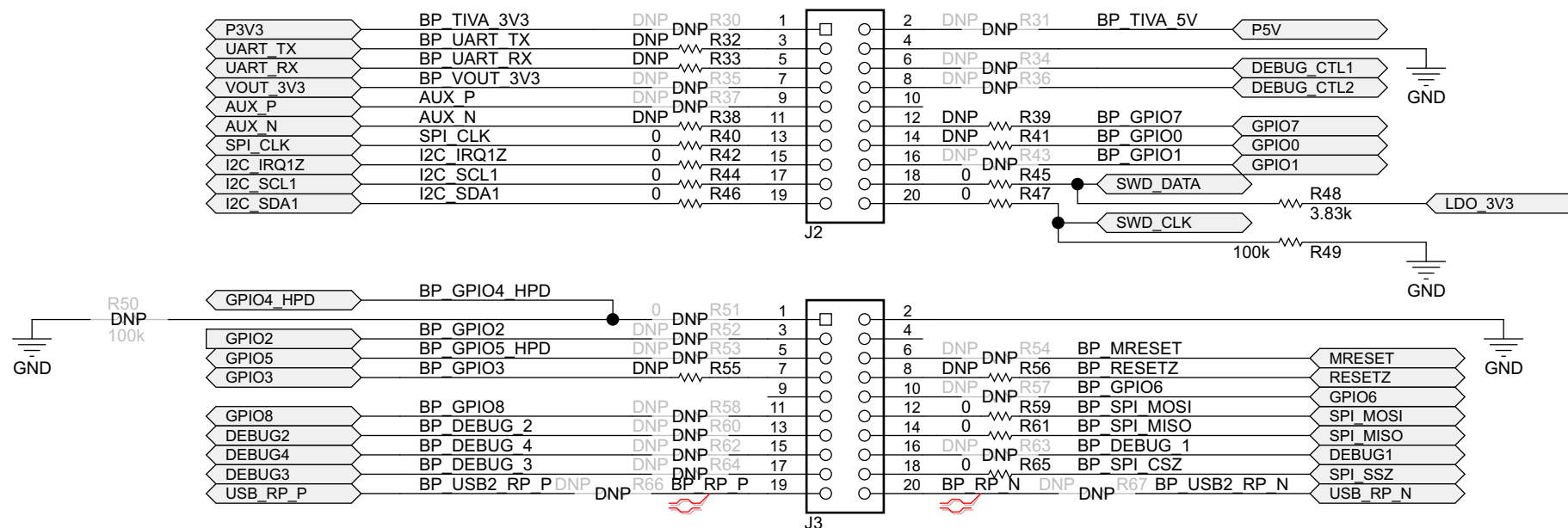
Figure 29. TPS65986EVM Booster Connector Block
