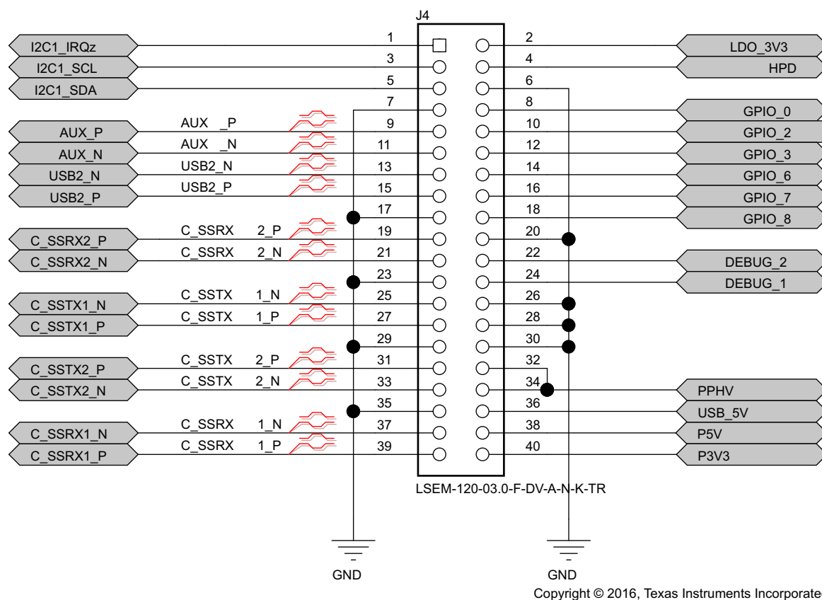
Figure 28. TPS65986EVM Inter PCB Block
