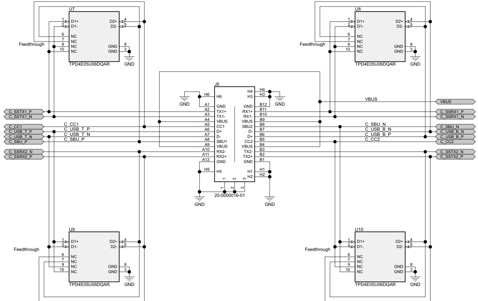
Figure 27. TPS65986EVM Type-C Block
