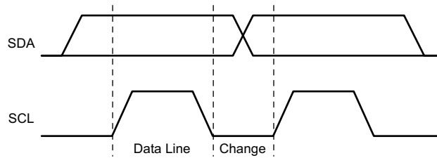
Figure 71. I 2 C Bit Transfer
