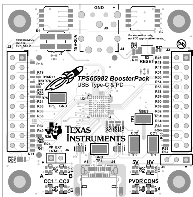
Figure 5. PCB Layer 1 (Top Layer)
