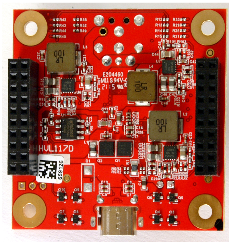
Figure 2. TPS65982-EVM (Bottom View)
