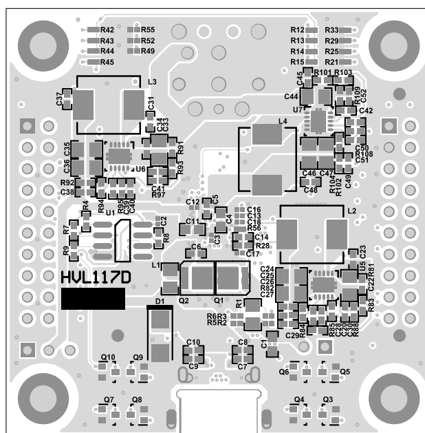
Figure 12. PCB Layer 6 (Component View)
