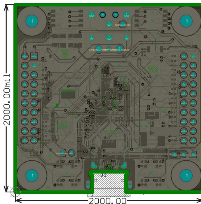
Figure 7. PCB Layer 2 (GND Plane)
