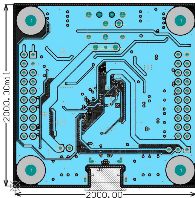
Figure 10. PCB Layer 5 (Inner Signal Layer 2)
