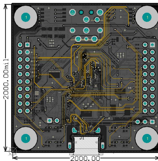
Figure 8. PCB Layer 3 (Inner Signal Layer 1)
