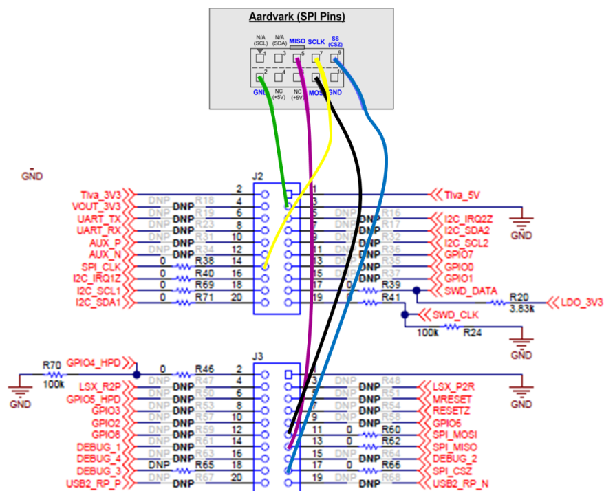
Figure 14. Aardvark Wired to SPI Pins
