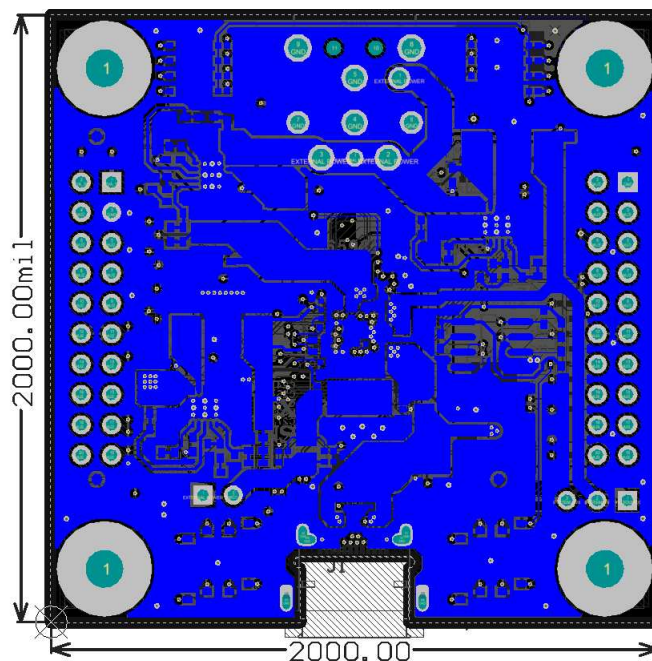
Figure 11. PCB Layer 6 (Bottom Layer)
