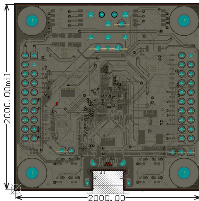
Figure 9. PCB Layer 4 (GND Plane)
