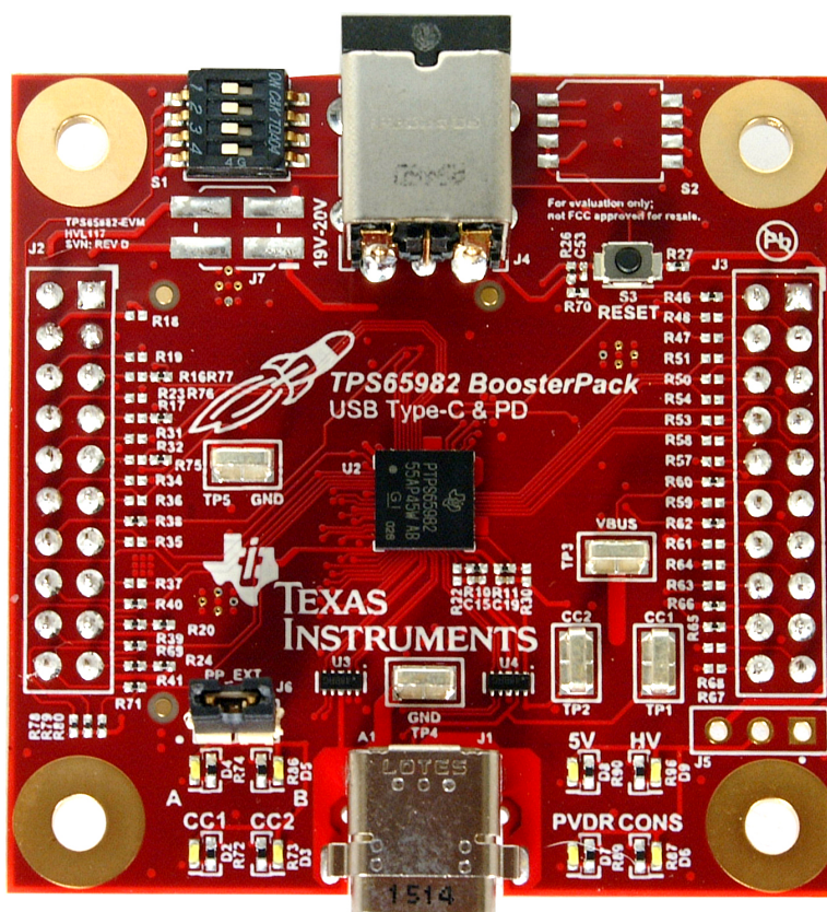
Figure 1. TPS65982-EVM (Top View)
